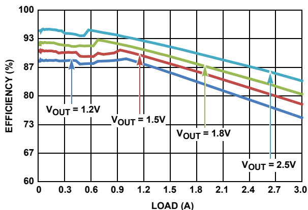
FIGURE 6. EFFICIENCY vs LOAD (ISL80031) f_{SW} = 1MHz , V_{IN} = 3.3V , PFM, T_A = +25^\circ C
