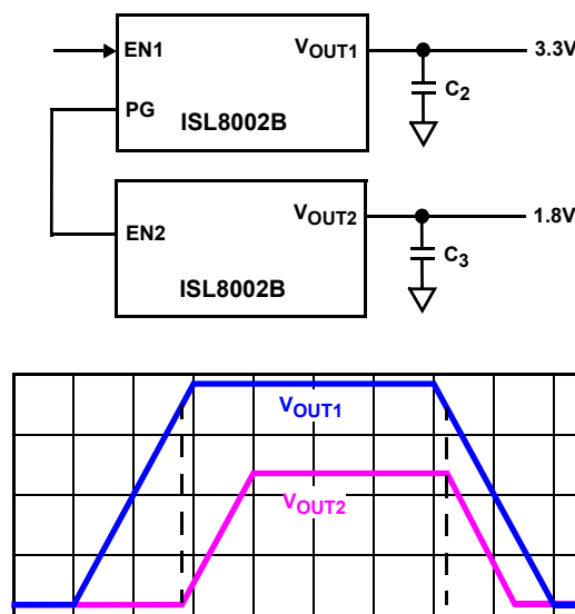
FIGURE 61. OUTPUT SEQUENCING
