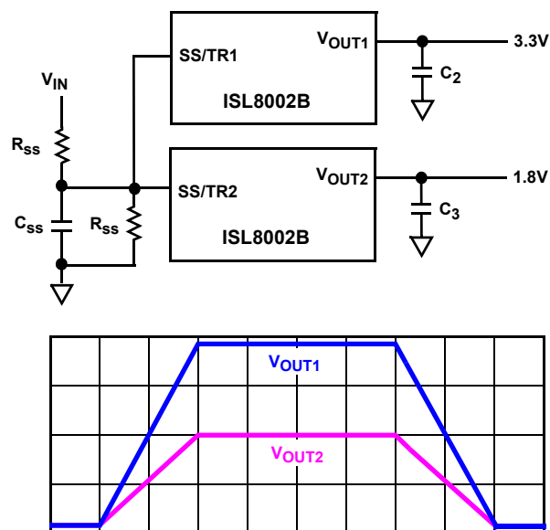
FIGURE 59. RATIOMETRIC START-UP
