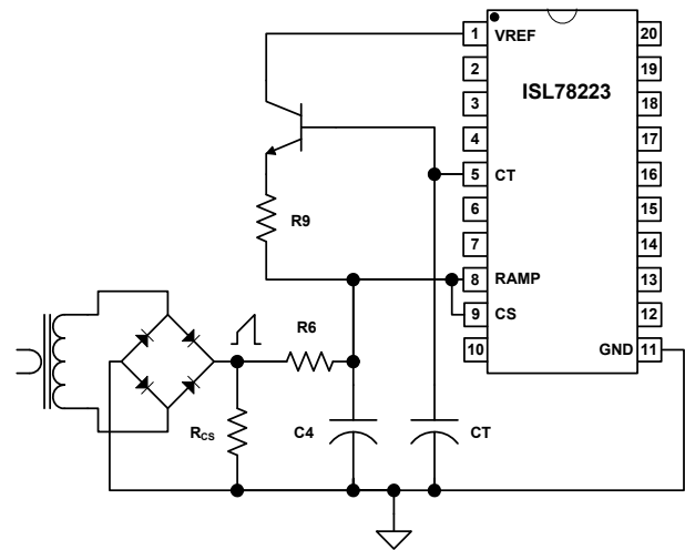
FIGURE 13. ADDING SLOPE COMPENSATION USING CT
