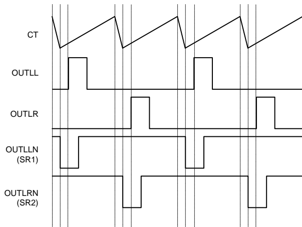
FIGURE 23. WAVEFORM TIMING WITH PWM OUTPUTS DELAYED, 0\text{V} < V_{ADJ} < 2.425\text{V}
