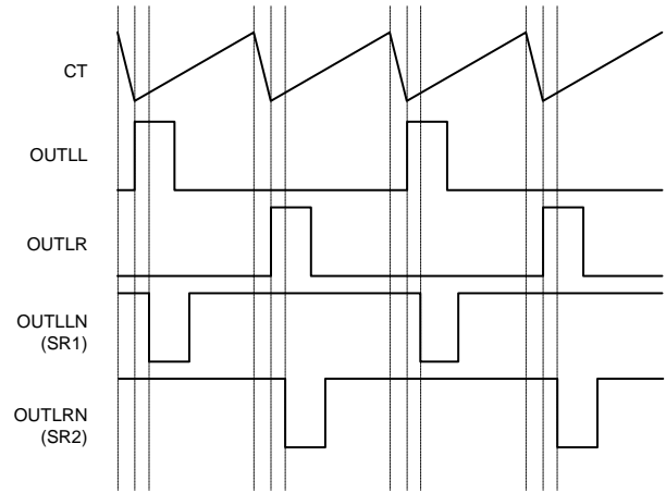
FIGURE 24. WAVEFORM TIMING WITH SR OUTPUTS DELAYED, 2.575\text{V} < V_{ADJ} < 5.00\text{V}
