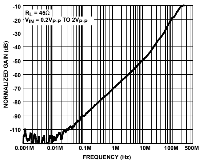
FIGURE 15. CROSSTALK
