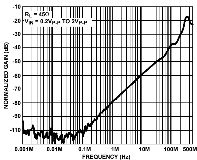
FIGURE 14. OFF-ISOLATION
