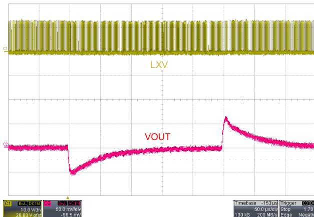
Figure 49. 12V_{IN} , 3.3V_{OUT} 500kHz, 2A Load Transient R_{SLOPE} = 44.2k\Omega , R_{COMP} = 14k\Omega , C_{COMP} = 3900pF , L_{OUT} = 4.7\mu H , C_{OUT} = 144\mu F
