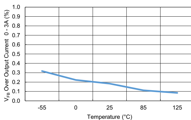
Figure 26. V_{FB} Over Output Current vs Temperature
