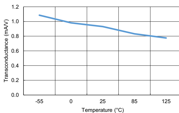
Figure 28. External Compensation Loop Error Amp Transconductance vs Temperature
