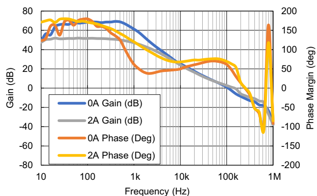
Figure 45. Ext Comp Gain/Phase BODE Plot, 3.3V IN , 1.0V OUT , 1MHz, R_{SLOPE} = 34.8k\Omega , R_{COMP} = 14k\Omega , C_{COMP} = 1200pF , L_{OUT} = 0.82\mu H , C_{OUT} = 172\mu F
