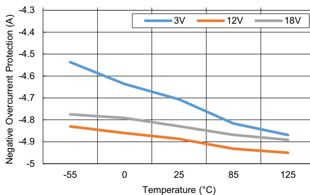
Figure 22. Negative Current Protection vs Temperature
