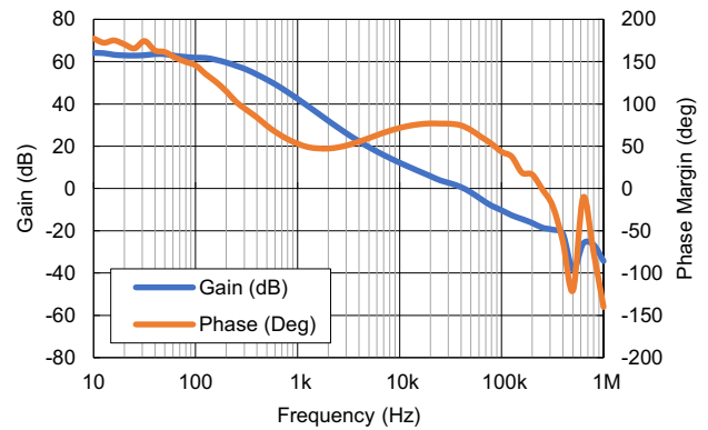
Figure 48. Internal Comp Gain/Phase BODE Plot, 12V_{IN} , 3.3V_{OUT} , 500kHz , I_{OUT} = 1.5A L_{OUT} = 4.7\mu H , C_{OUT} = 144\mu F
