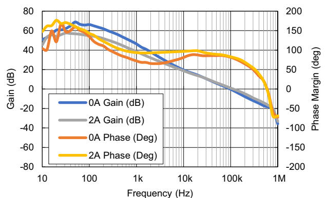
Figure 46. Int Comp Gain/Phase BODE Plot, 3.3V IN , 1.0V OUT , 1MHz, L_{OUT} = 0.82\mu H , C_{OUT} = 172\mu F
