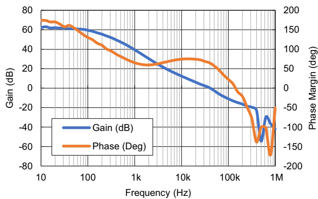
Figure 47. External Comp Gain/Phase BODE Plot, 12V_{IN} , 3.3V_{OUT} , 500kHz , I_{OUT} = 1.5A R_{SLOPE} = 44.2k\Omega , R_{COMP} = 14k\Omega , C_{COMP} = 3900pF , L_{OUT} = 4.7\mu H , C_{OUT} = 144\mu F
