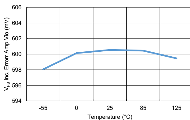
Figure 24. FB Voltage vs Temperature
