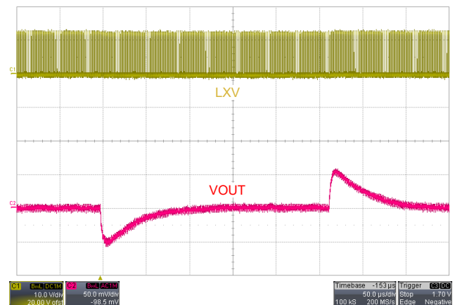
Figure 50. 12V_{IN} , 3.3V_{OUT} , 500kHz, 2A Load Transient (Internal Compensation), L_{OUT} = 4.7\mu H , C_{OUT} = 144\mu F
