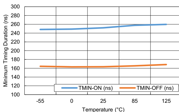
Figure 18. Minimum On-Time/Off-Time vs Temperature
