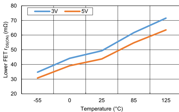
Figure 20. Lower FET r_{DS(ON)} vs Temperature
