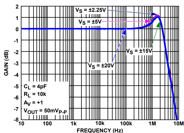
FIGURE 34. GAIN vs FREQUENCY vs SUPPLY VOLTAGE
