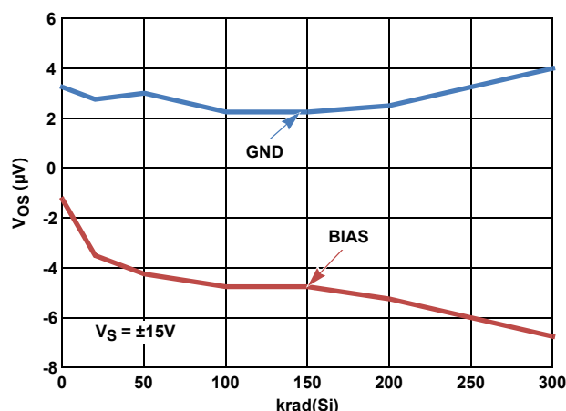
FIGURE 2. V_{OS} SHIFT vs HIGH DOSE RATE RADIATION
