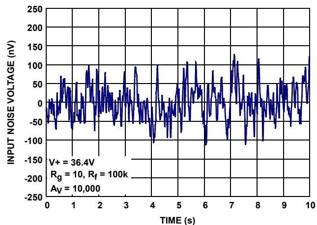
FIGURE 23. INPUT NOISE VOLTAGE 0.1Hz TO 10Hz
