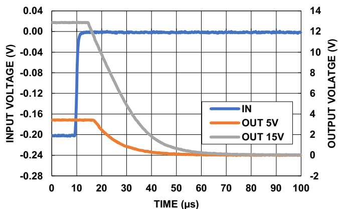
FIGURE 39. POSITIVE OUTPUT OVERLOAD RESPONSE TIME, V_S = \pm 5V, \pm 15V , R_L = 2k , C_L = 4pF , A_V = -100 , R_f = 100k , R_g = 1k , V_{IN} = 200mV_{p-p}
