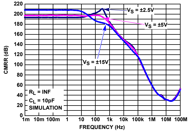
FIGURE 28. CMRR vs FREQUENCY, V_S = \pm 2.25V, \pm 5V, \pm 15V
