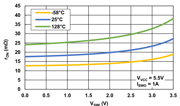
Figure 2. r_{ON} vs V_{SWI} vs Temperature
