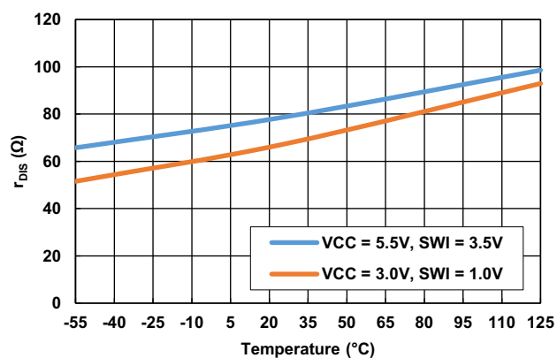
Figure 41. r_{DS} vs V_{SWI} vs Temperature
