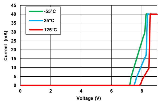
Figure 22. V_{CC} , SWI , SWO , ON , DON Breakdown Voltage
