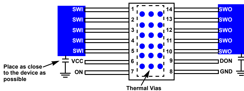
Figure 47. Layout Recommendations
