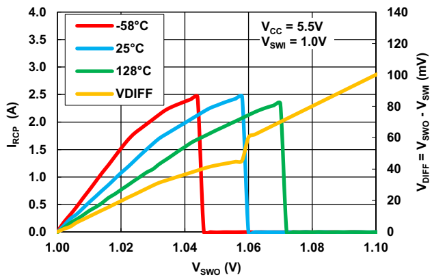
Figure 35. I_{RCP} Enter vs V_{SWO} vs Temperature
