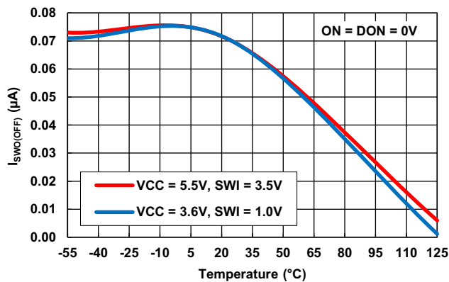
Figure 19. I_{SWO(OFF)} vs Temperature
