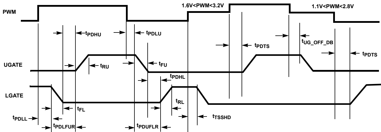
FIGURE 2. TIMING DIAGRAM
