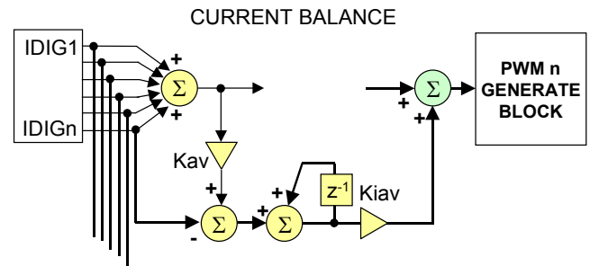
FIGURE 10. CURRENT BALANCE
