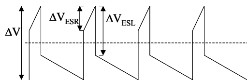
FIGURE 44. CONTRIBUTIONS OF ESR AND ESL OF OUTPUT CAPACITOR TO OUTPUT VOLTAGE RIPPLE
