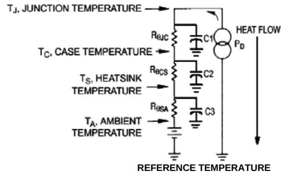
FIGURE 37. THERMAL RESISTIVITY MODELING
