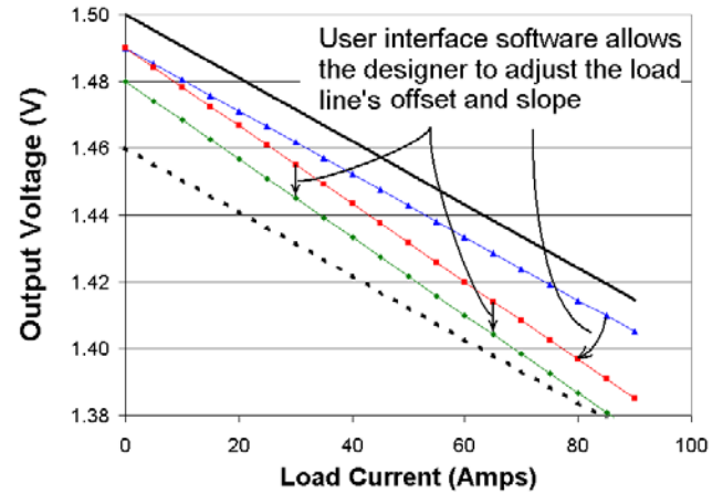
FIGURE 7. USER INTERFACE LOAD LINE ADJUSTMENTS
