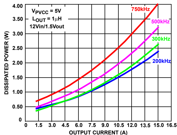
FIGURE 9. ISL6571 POWER DISSIPATION vs CURRENT AT 200kHz, 300kHz, 500kHz, 750kHz
