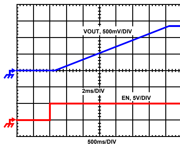
FIGURE 12. SOFT-START WAVEFORMS WITH AN UN-BIASED OUTPUT. FSW = 500kHz
