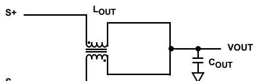
FIGURE 20A. CURRENT DOUBLER FILTER
