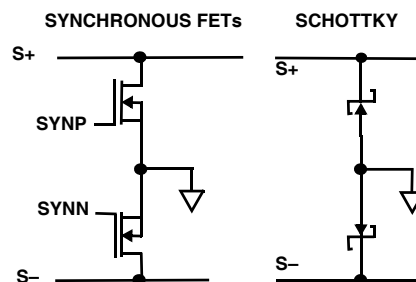
FIGURE 17A. CURRENT DOUBLER RECTIFIERS
