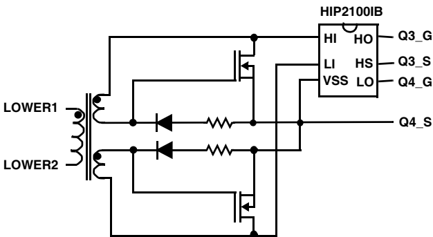
FIGURE 23B. PUSH-PULL HIGH CURRENT DRIVERS
