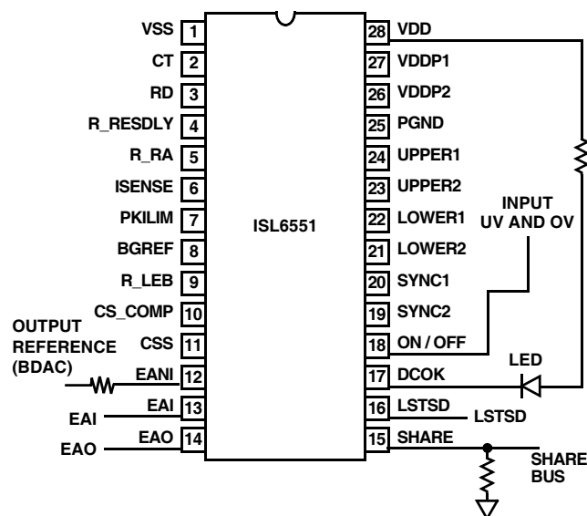
FIGURE 21. ISL6551IREC CONTROLLER
