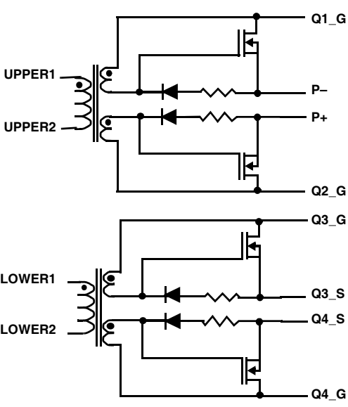
FIGURE 24B. FULL BRIDGE MEDIUM CURRENT DRIVERS
