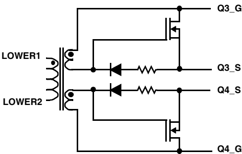
FIGURE 23A. PUSH-PULL MEDIUM CURRENT DRIVERS
