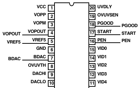
FIGURE 19. ISL6550
