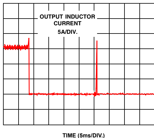
FIGURE 1. OVERCURRENT OPERATION
