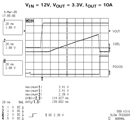
FIGURE 13. PG00D DELAY
