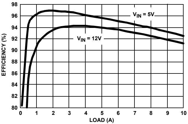
FIGURE 4. EFFICIENCY vs. LOAD CURRENT (VOUT = 3.3V)
