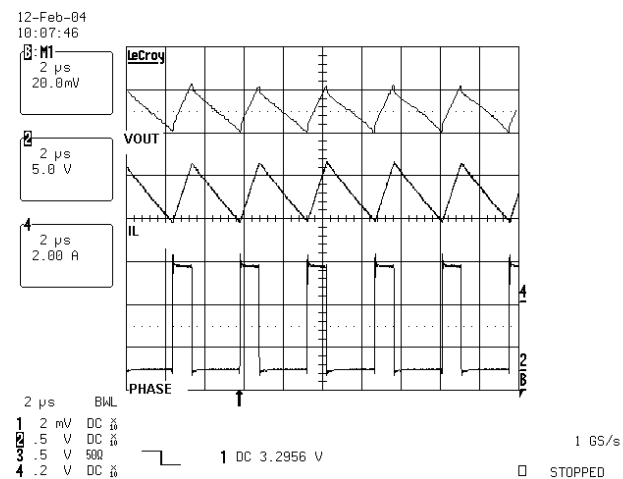
FIGURE 5. PWM WAVEFORMS
