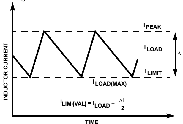
FIGURE 69. "VALLEY" CURRENT LIMIT THRESHOLD POINT
