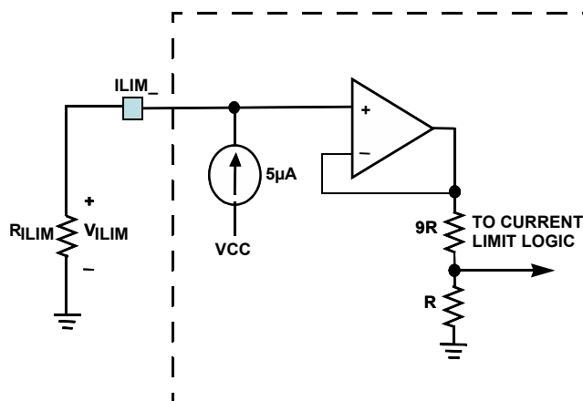
FIGURE 70. CURRENT LIMIT BLOCK DIAGRAM
