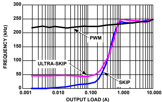
FIGURE 21. V_{OUT2} = 1.05V FREQUENCY vs LOAD
