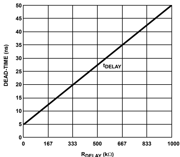
FIGURE 9. ISL6208A PROGRAMMABLE DEAD-TIME vs DELAY RESISTOR
