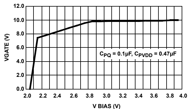
FIGURE 6. V_GATE vs V_BIAS
