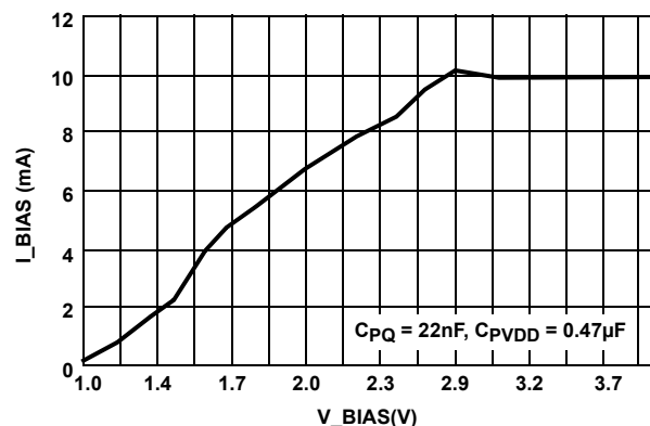
FIGURE 3. I_BIAS vs V_BIAS
