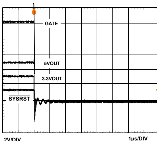
FIGURE 8. SYSRST LOW TO OUTPUT LATCH-OFF
