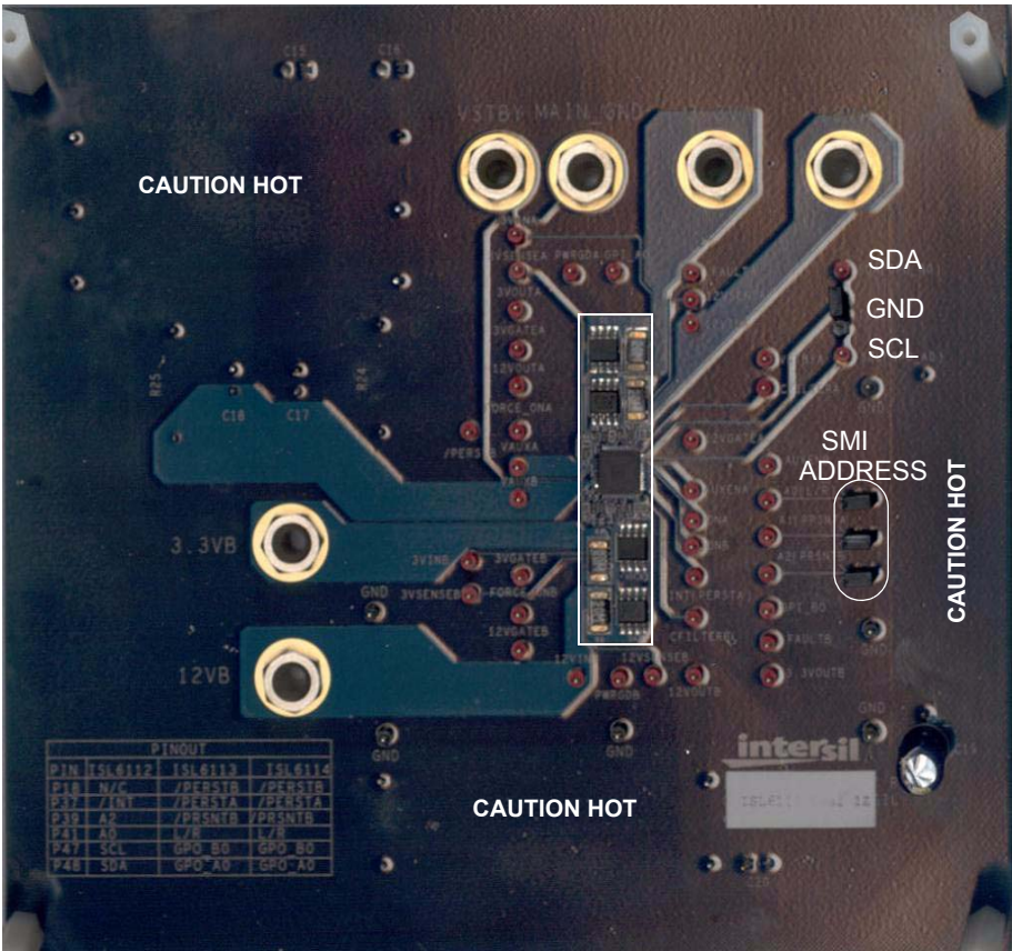
FIGURE 36. ISL6112EVAL1Z BOARD PHOTO
