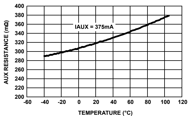
FIGURE 8. AUX r_{DS(ON)} vs TEMPERATURE
