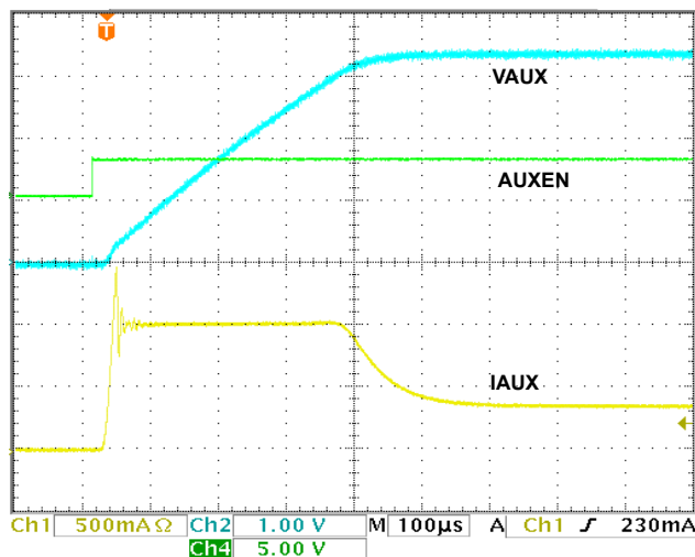
FIGURE 17. VAUX TURN-ON R_{\text{LOAD}} = 10\Omega , C_{\text{LOAD}} = 100\mu\text{F}
