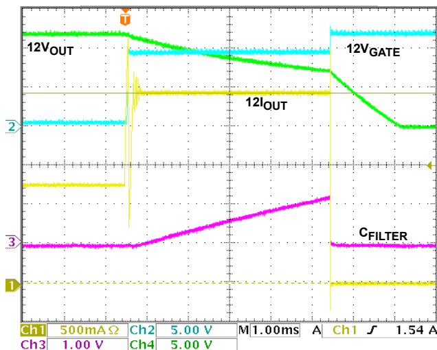
FIGURE 28. 12VMAIN CR AND SHUT-DOWN
