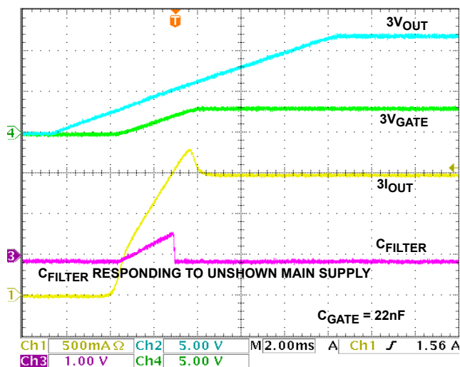
FIGURE 19. 3VMAIN START-UP R_{\text{LOAD}} = 2\Omega , C_{\text{LOAD}} = 470\mu\text{F}
