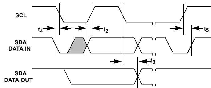
FIGURE 31. SMBUS TIMING
