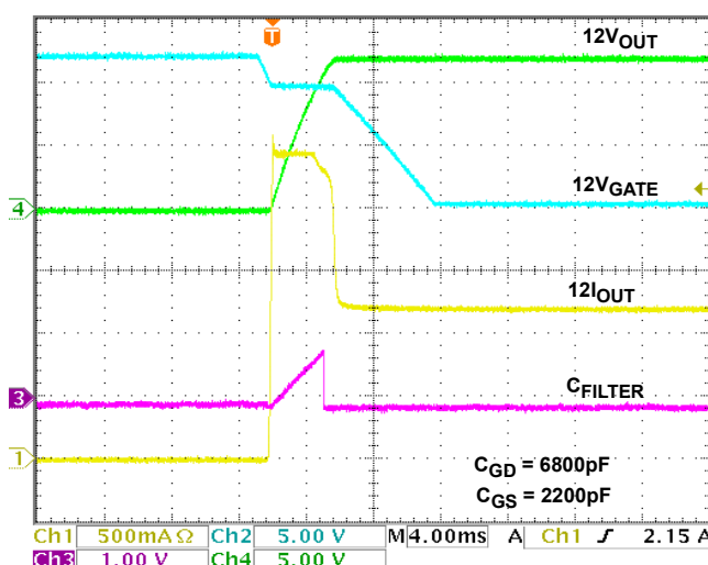
FIGURE 20. 12VMAIN START-UP R_{\text{LOAD}} = 10\Omega , C_{\text{LOAD}} = 470\mu\text{F}
