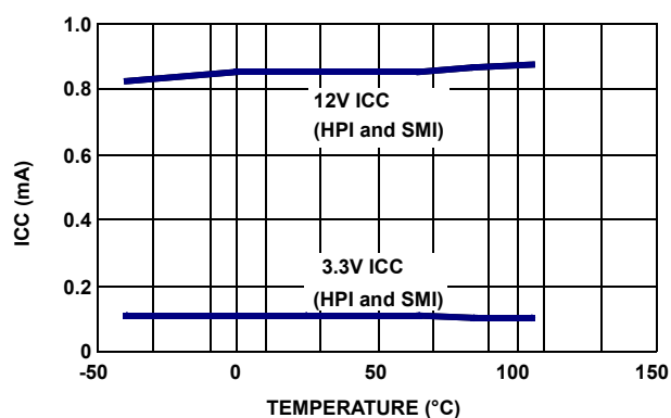
FIGURE 4. ICC CURRENT vs TEMPERATURE
