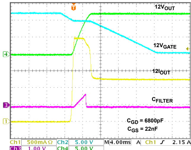
FIGURE 18. 12VMAIN START-UP R_{\text{LOAD}} = 10\Omega , C_{\text{LOAD}} = 470\mu\text{F}
