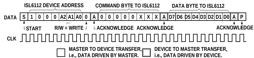
FIGURE 33. WRITE_BYTE PROTOCOL
