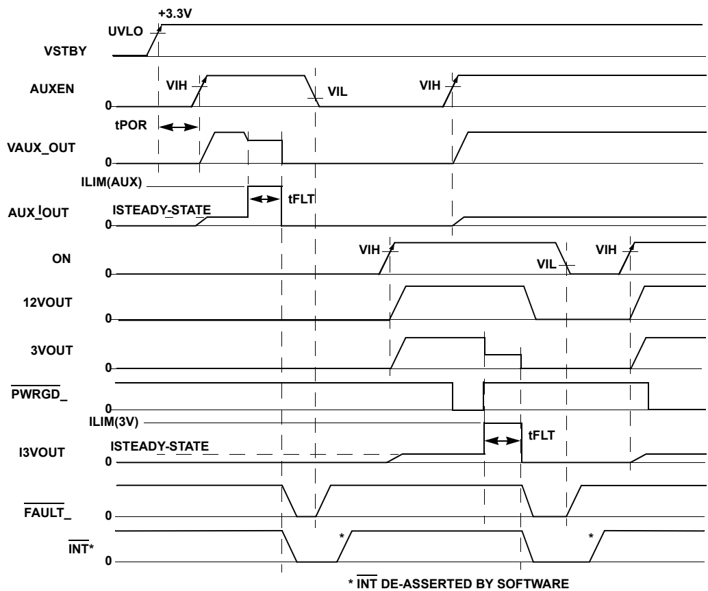
FIGURE 32. HOT-PLUG INTERFACE OPERATION
