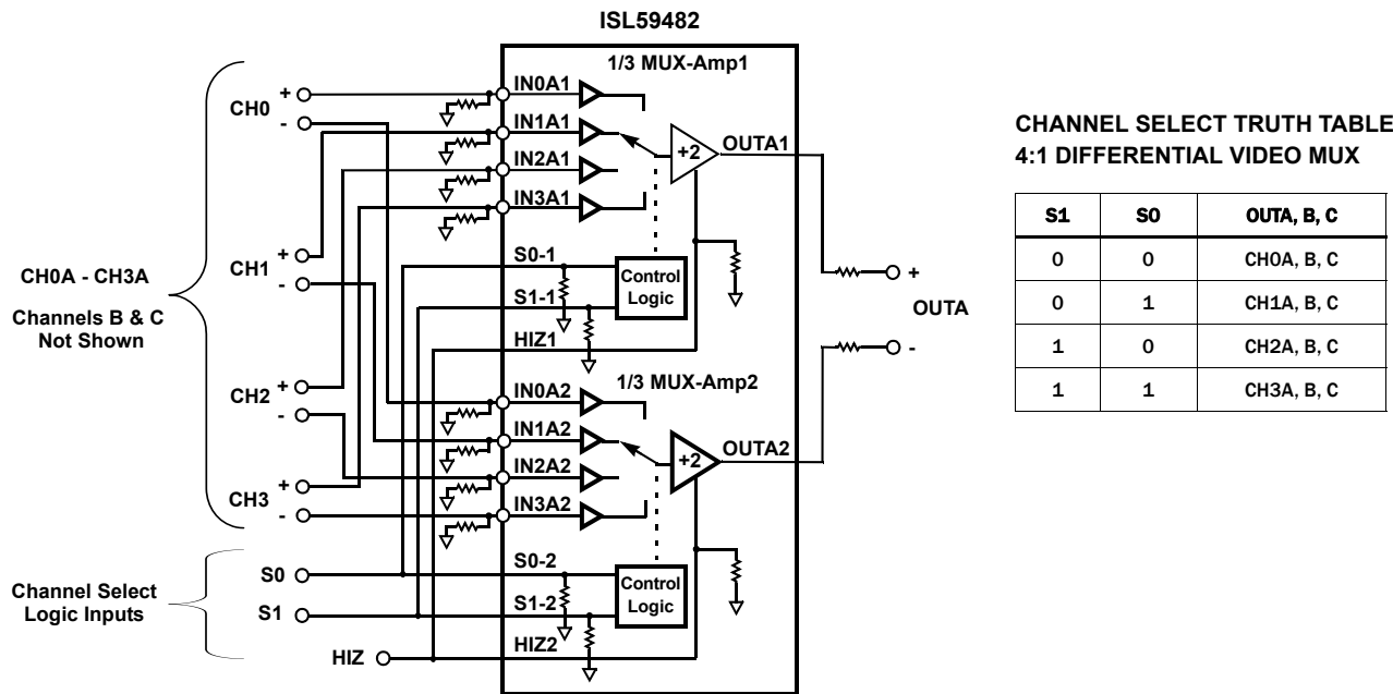
FIGURE 30. APPLICATION CIRCUIT FOR 4:1 RGB DIFFERENTIAL VIDEO MUX
