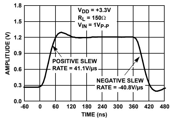
FIGURE 12. SLEW RATE
