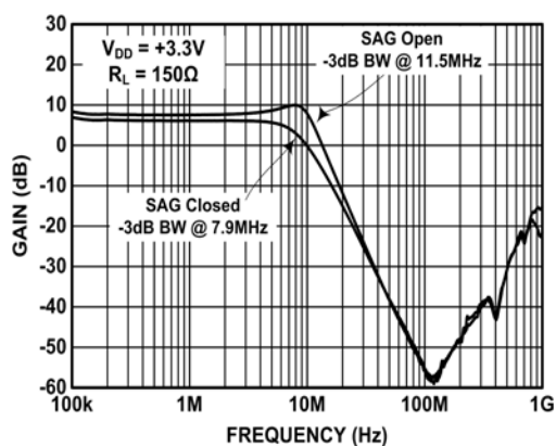
FIGURE 3. GAIN vs FREQUENCY -3dB
