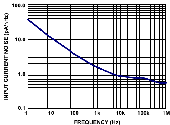
FIGURE 11. INPUT REFERRED NOISE CURRENT vs FREQUENCY
