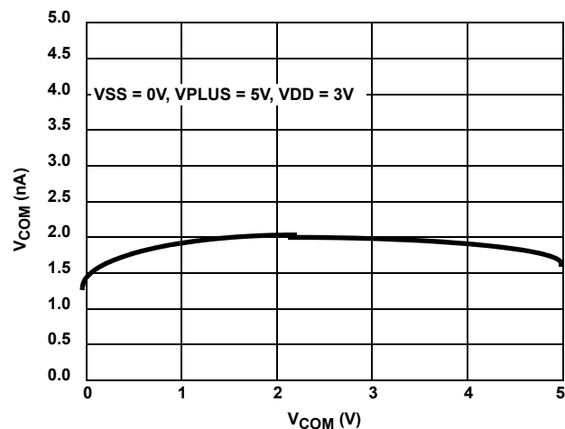
FIGURE 16. ON-LEAKAGE vs SWITCH VOLTAGE
