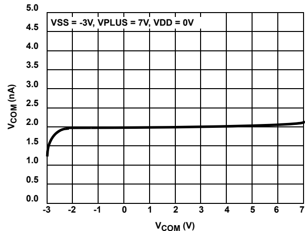
FIGURE 17. ON-LEAKAGE vs SWITCH VOLTAGE
