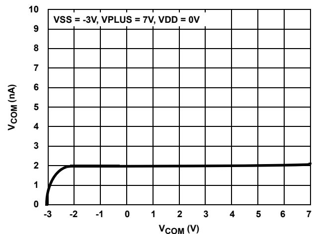
FIGURE 23. OFF-LEAKAGE vs SWITCH VOLTAGE
