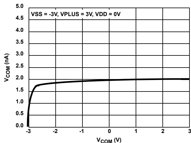
FIGURE 21. OFF-LEAKAGE vs SWITCH VOLTAGE
