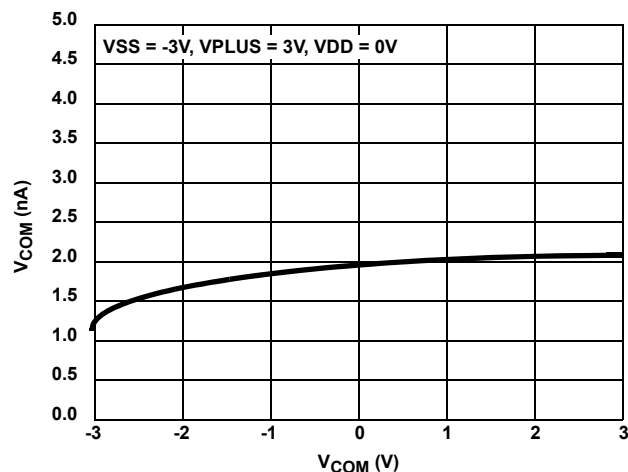
FIGURE 15. ON-LEAKAGE vs SWITCH VOLTAGE
