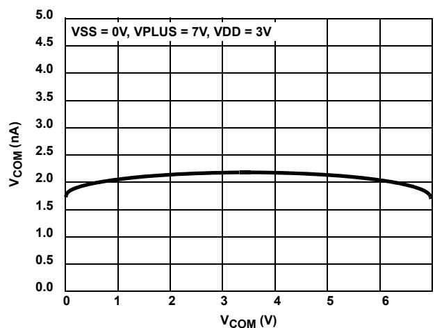
FIGURE 18. ON-LEAKAGE vs SWITCH VOLTAGE
