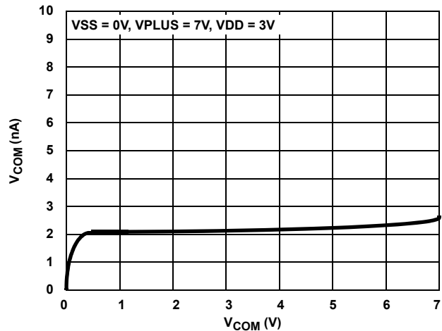
FIGURE 24. OFF-LEAKAGE vs SWITCH VOLTAGE
