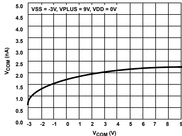
FIGURE 19. ON-LEAKAGE vs SWITCH VOLTAGE
