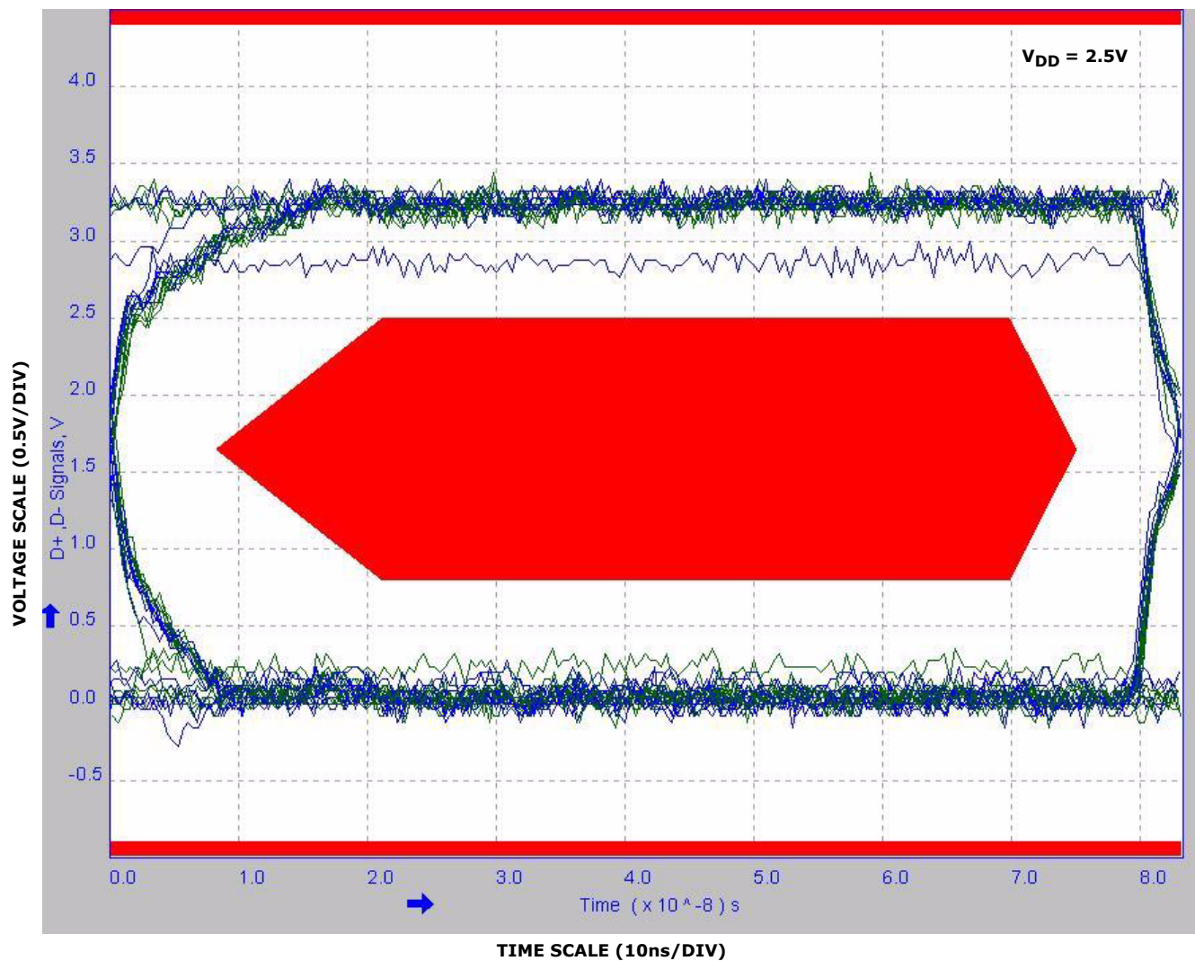
FIGURE 14. EYE PATTERN: 12Mbps WITH SWITCHES IN THE SIGNAL PATH
