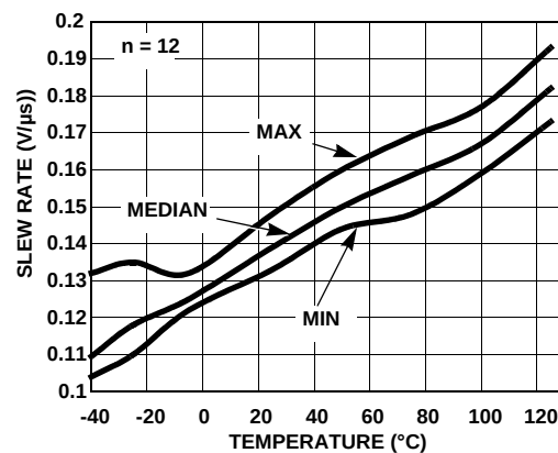
FIGURE 34. -SLEW RATE vs TEMPERATURE V_S = \pm 2.5V , INPUT = \pm 0.75V A_V = 2
