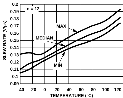
FIGURE 33. +SLEW RATE vs TEMPERATURE V_S = \pm 2.5V , INPUT = \pm 0.75V A_V = 2
