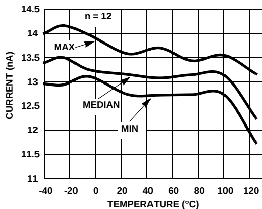
FIGURE 31. I_{IL} (EN) vs TEMPERATURE V_S = \pm 2.5V
