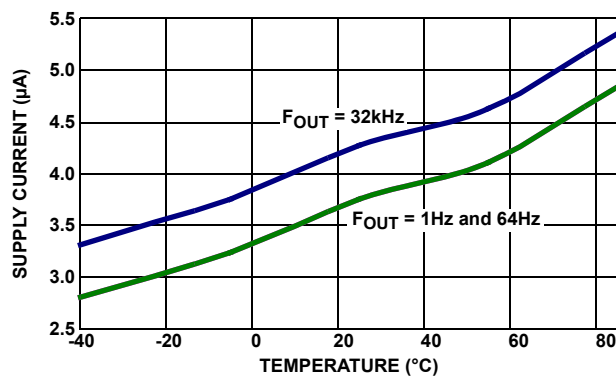
FIGURE 7. I_{DD} vs TEMPERATURE, 3 DIFFERENT F_{OUT}
