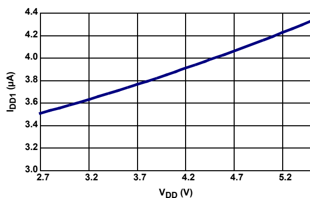
FIGURE 5. I_{DD1} vs V_{DD}
