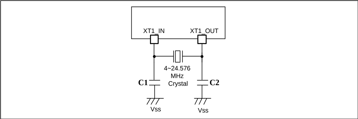
Figure 6.4-2 HXT Typical Crystal Application Circuit
