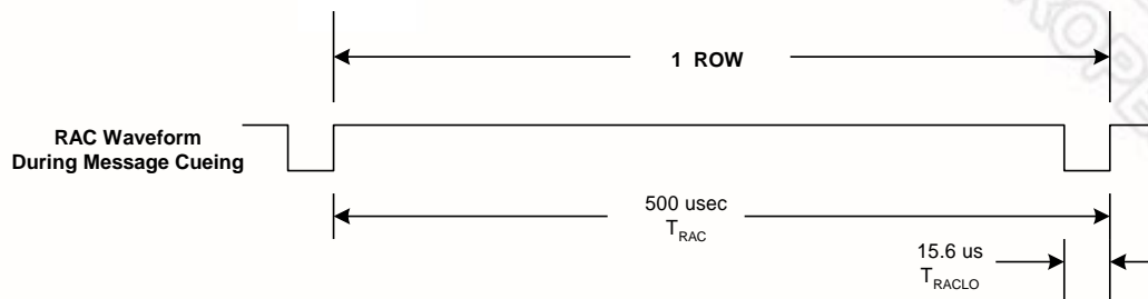
RAC Waveform During Digital Erase
