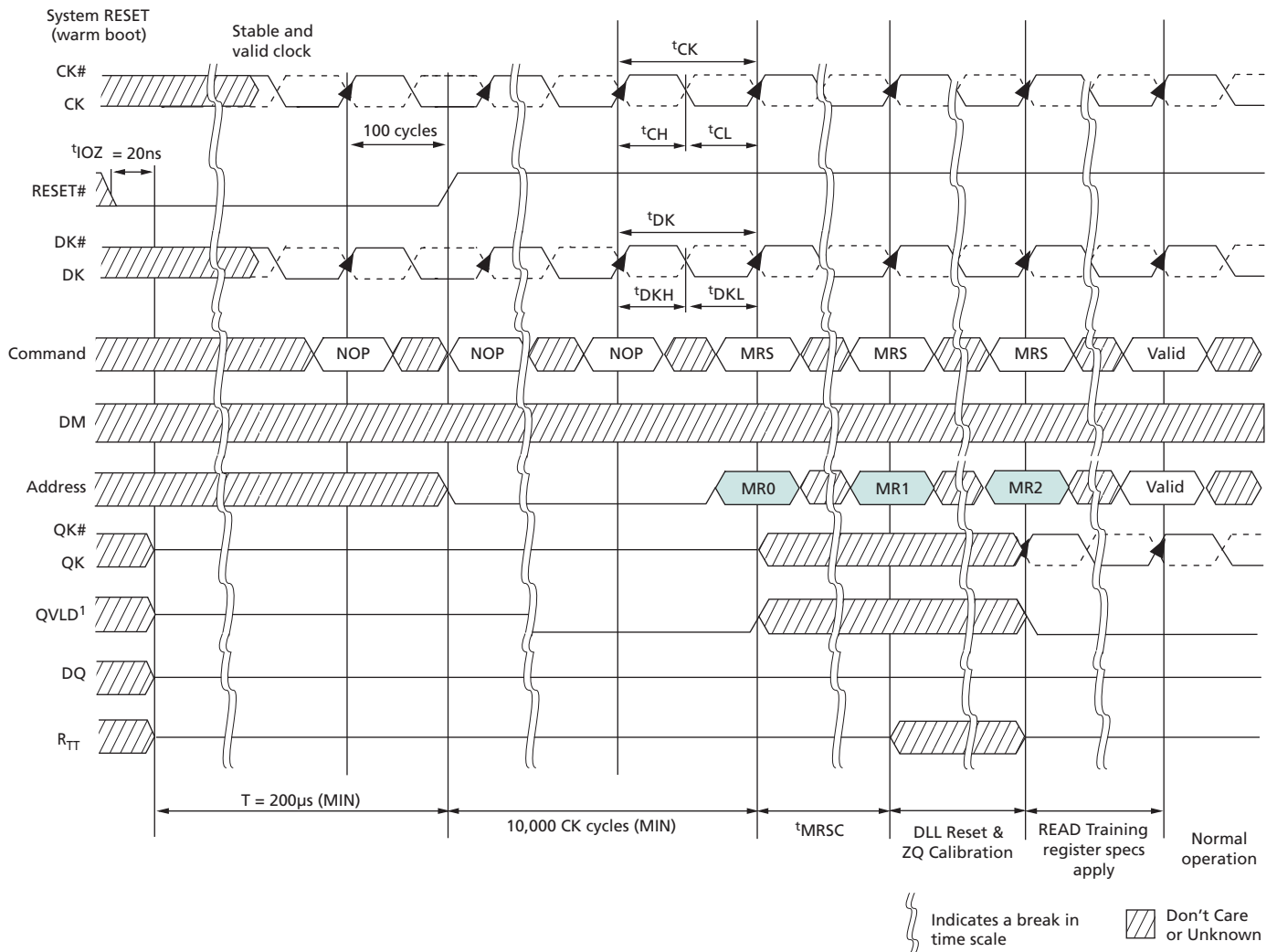
Figure 58: RESET Sequence
