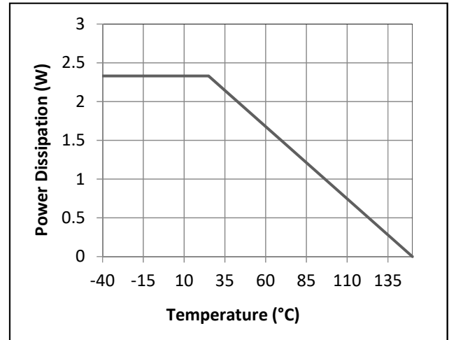
Figure 39 Dissipation Curve
