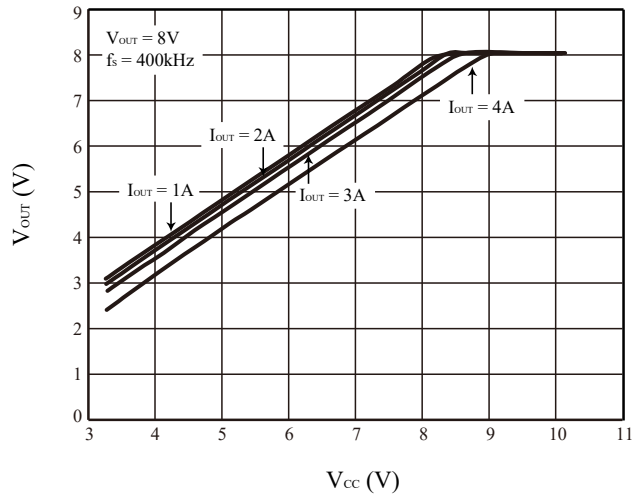
Figure 20 V_{OUT} vs. V_{CC}
