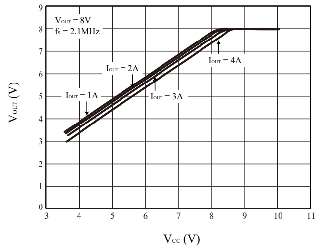
Figure 15 V_{OUT} vs. V_{CC}
