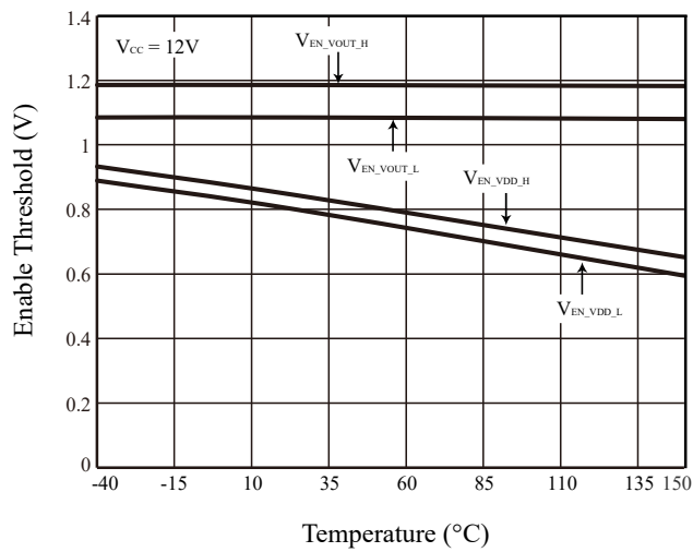
Figure 4 Enable Threshold vs. Temperature
