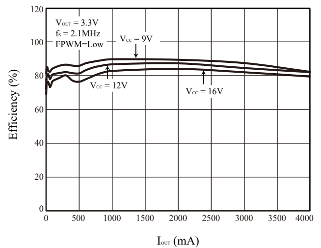
Figure 11 Efficiency vs. I_{OUT}
