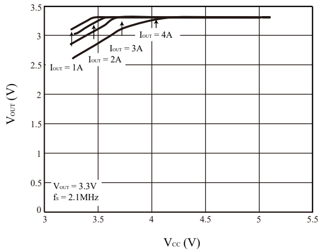
Figure 16 V_{OUT} vs. V_{CC}
