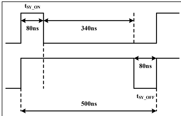
Figure 33 2MHz SYNC Application Example
