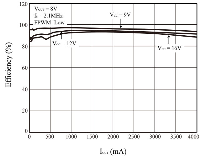
Figure 9 Efficiency vs. I_{OUT}
