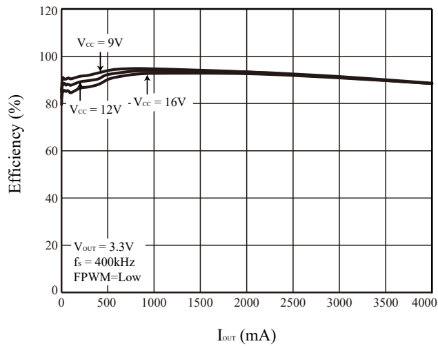
Figure 14 Efficiency vs. I_{OUT}
