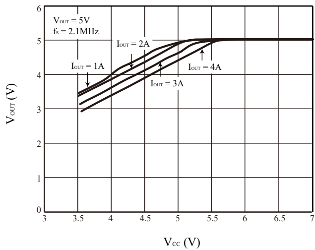
Figure 18 V_{OUT} vs. V_{CC}
