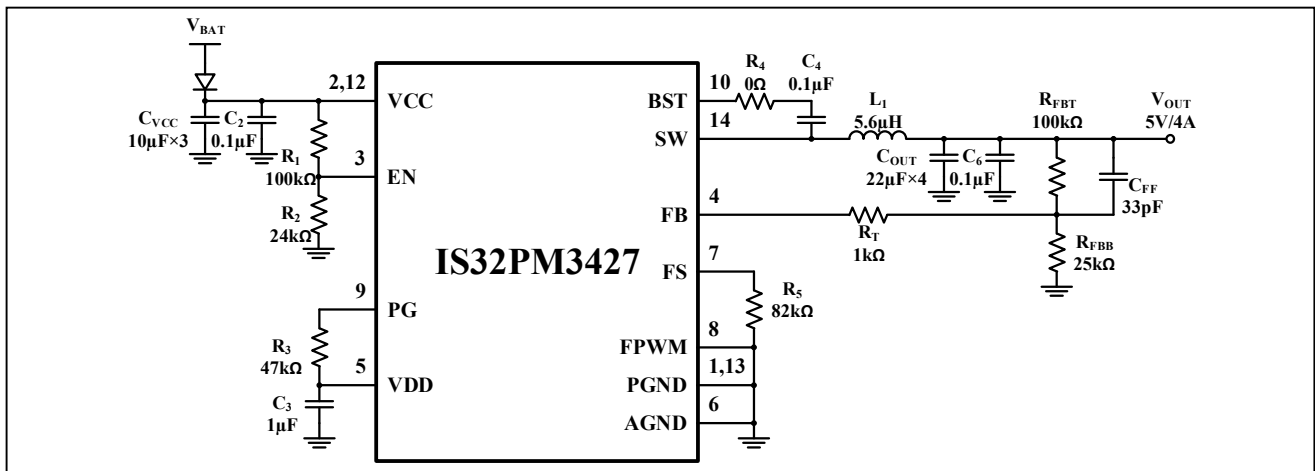
Figure 37 f_{SW}=400kHz 5V/4A Output Application Example
