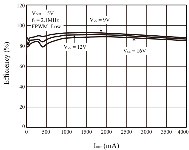
Figure 10 Efficiency vs. I_{OUT}
