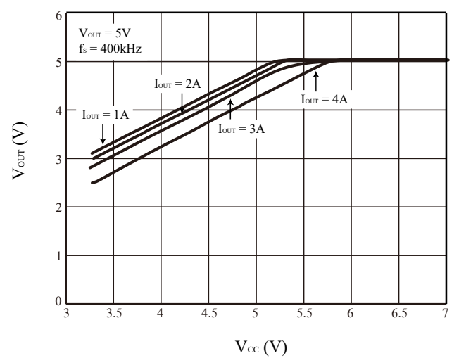
Figure 19 V_{OUT} vs. V_{CC}
