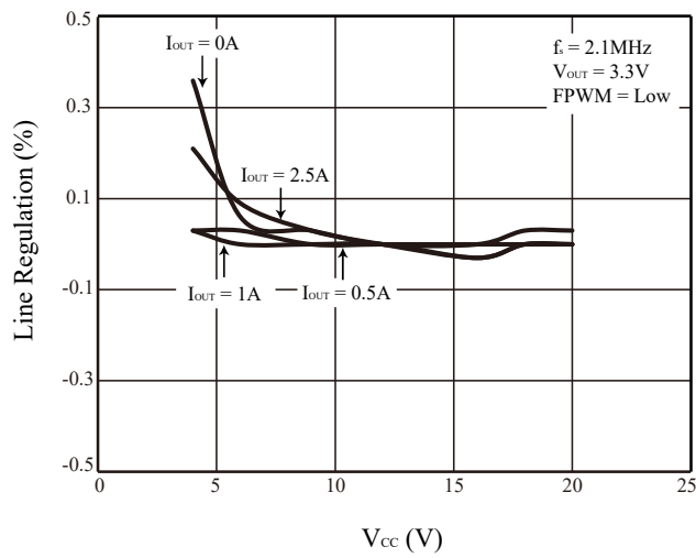
Figure 22 Line Regulation
