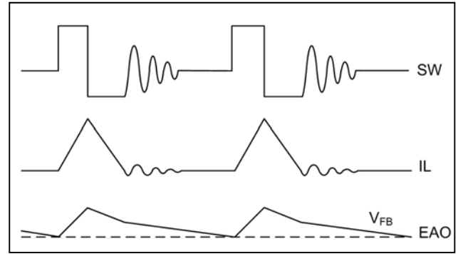
Figure 29 PFM Operation Mode at Light-load
