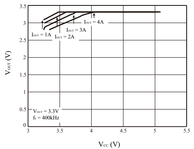
Figure 17 V_{OUT} vs. V_{CC}
