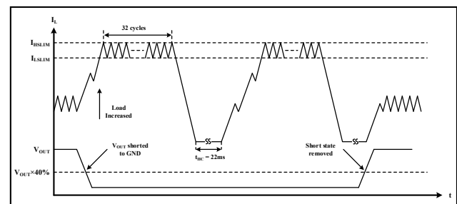
Figure 30 Hiccup Mode
