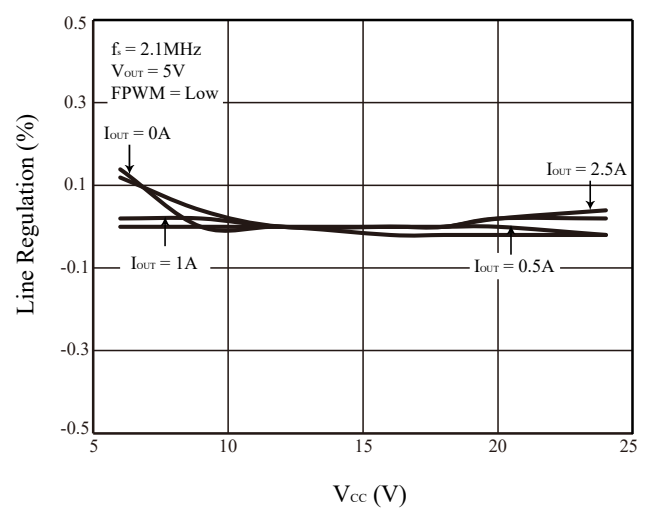
Figure 23 Line Regulation
