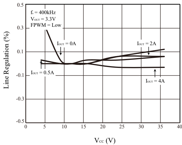
Figure 24 Line Regulation
