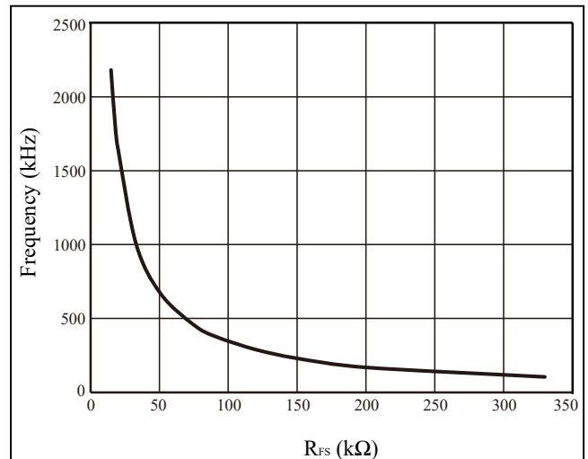
Figure 32 Frequency vs. R_{FS}
