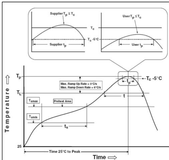
Figure 41 Classification Profile
