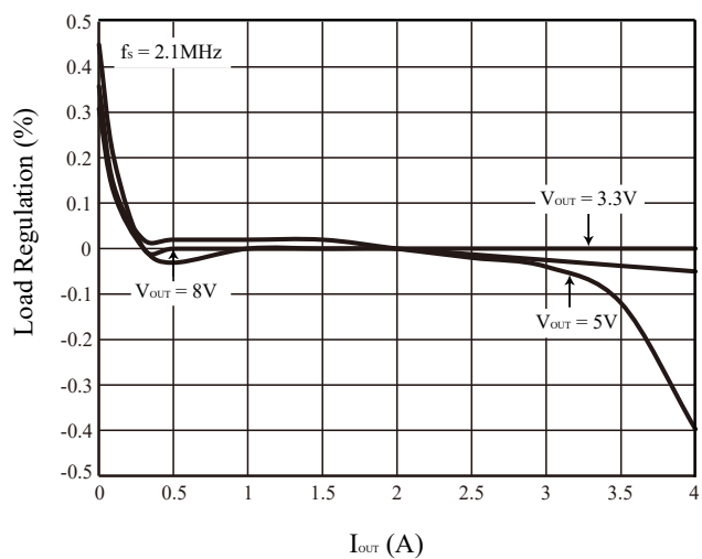
Figure 28 Load Regulation
