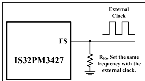
Figure 34 FS Pin Configuration
