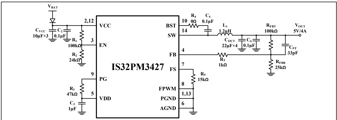
Figure 38 f_{SW}=2.1MHz 5V/4A Output Application Example
