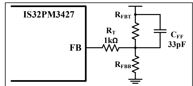
Figure 36 Feedback Network
