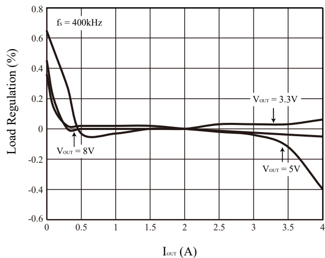
Figure 27 Load Regulation
