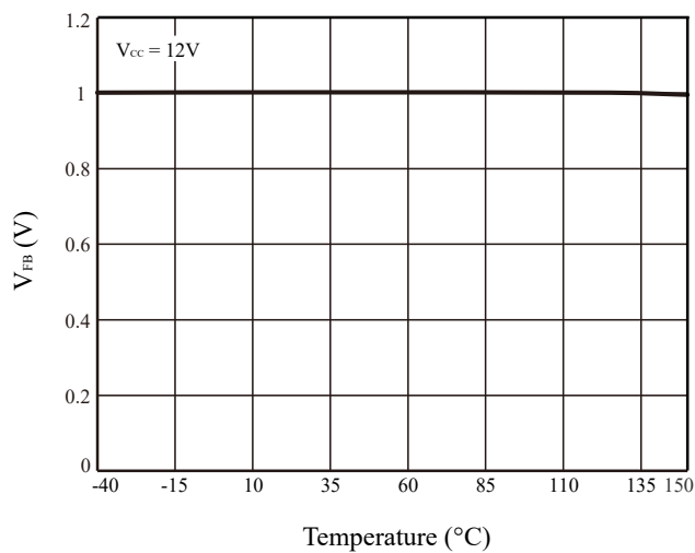
Figure 6 V_{FB} vs. Temperature
