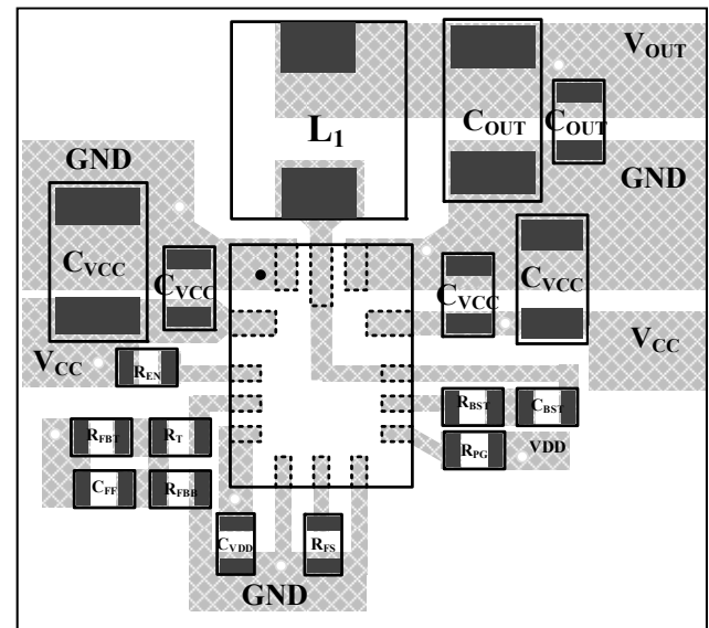
Figure 40 PCB Layout Example (Top Layer)
