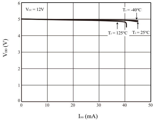
Figure 8 V_{DD} vs. I_{DD}
