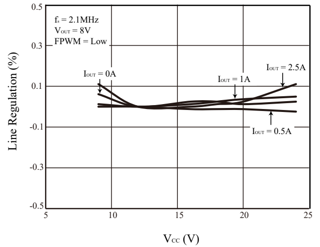
Figure 21 Line Regulation
