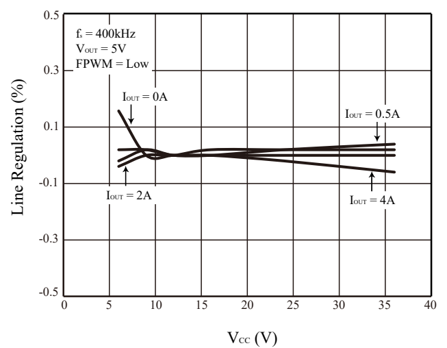
Figure 25 Line Regulation
