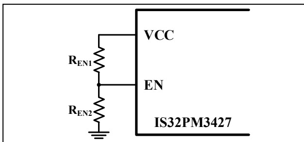
Figure 35 EN Configuration
