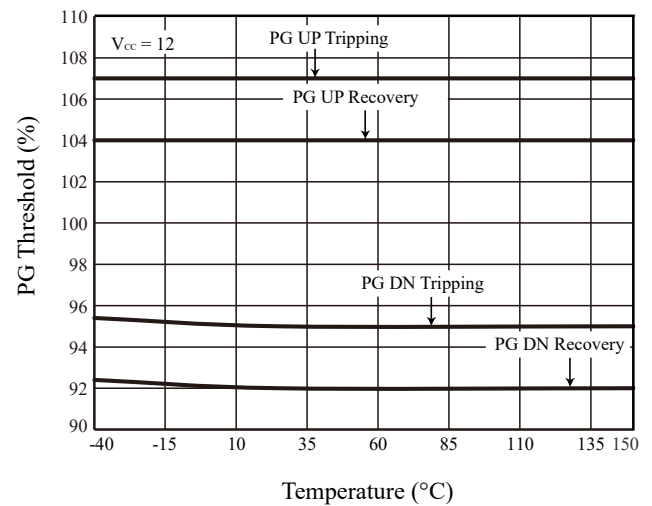
Figure 5 PG Threshold vs. Temperature
