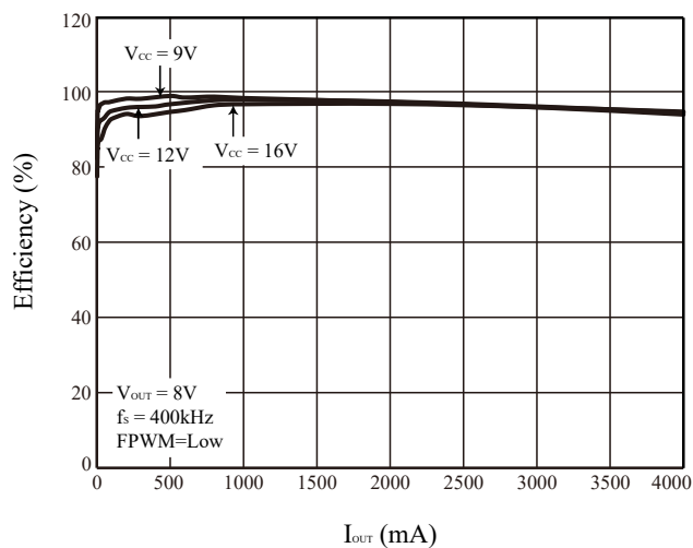
Figure 12 Efficiency vs. I_{OUT}
