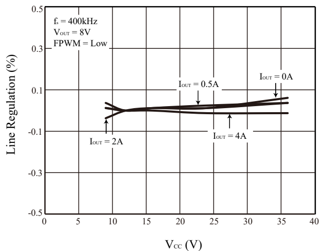
Figure 26 Line Regulation
