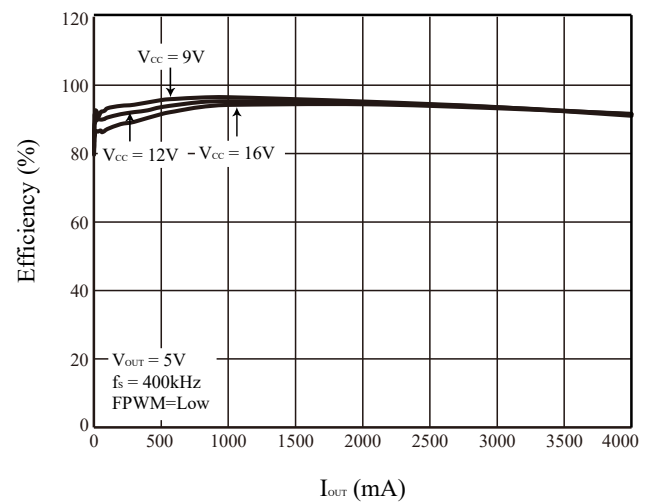
Figure 13 Efficiency vs. I_{OUT}
