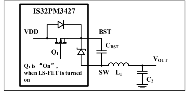
Figure 31 Bootstrap Charging Circuit
