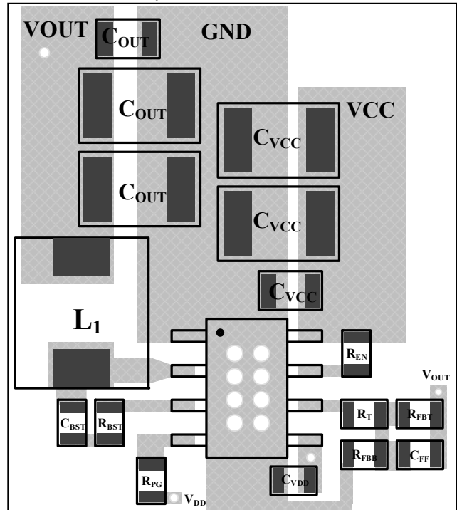
Figure 19 PCB Layout Example (Top Layer)
