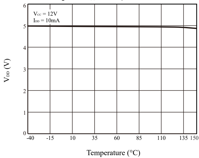
Figure 4 V_{DD} vs. Temperature
