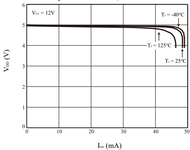
Figure 6 V_{DD} vs. I_{DD}
