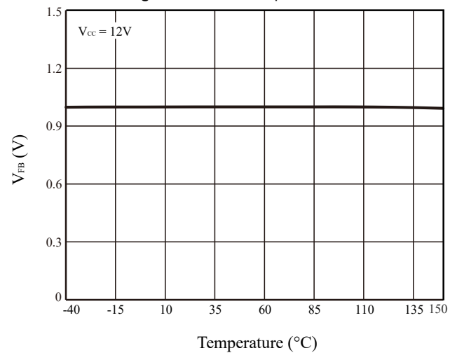
Figure 5 V_{FB} vs. Temperature
