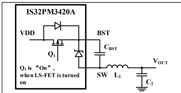
Figure 14 Bootstrap Charging Circuit
