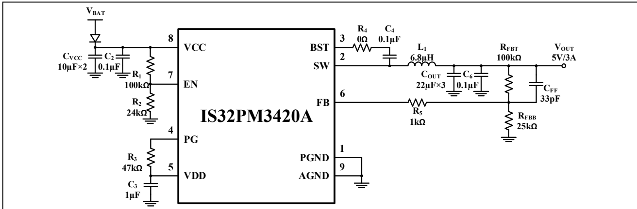
Figure 17 5V/3A Output Application Example
