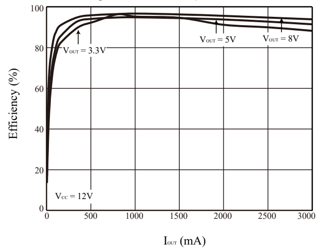
Figure 7 Efficiency vs. I_{OUT}
