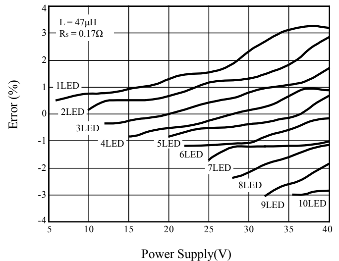
Figure 3 Output Current Error vs. Power Supply
