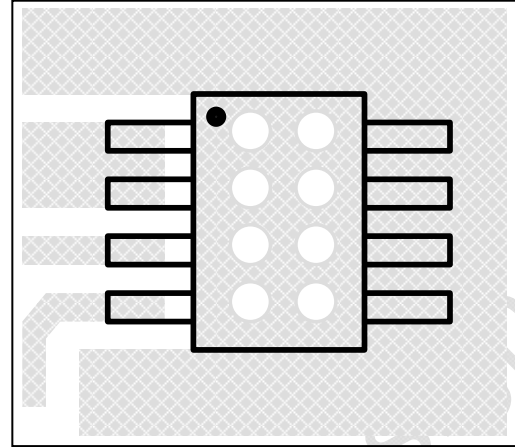
Figure 40 Board Via Layout For Thermal Dissipation
