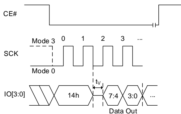
Figure 8.105 RDABR QPI Sequence (QE = 1)
