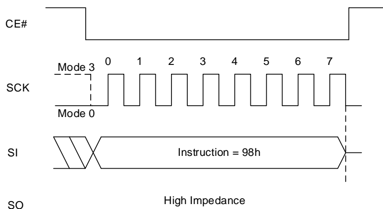
Figure 8.150 Gang Sector/Block Unlock Sequence
