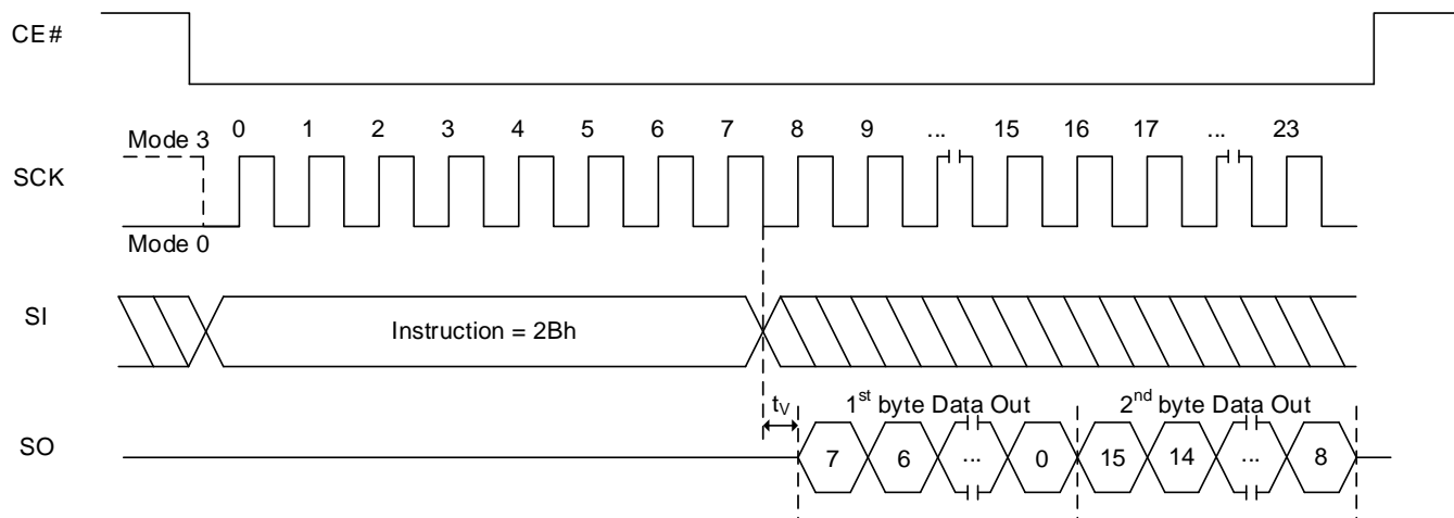
Figure 8.132 Read ASP Sequence
