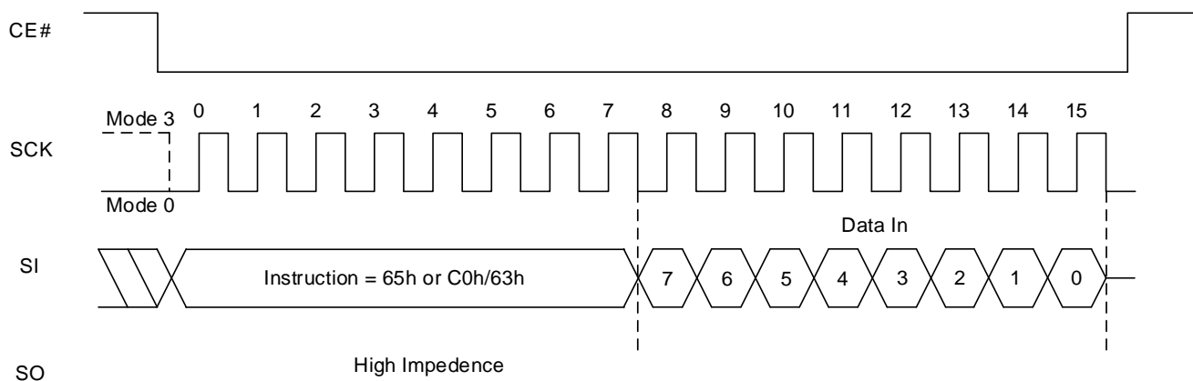
Figure 8.59 Set Read Parameters Sequence
