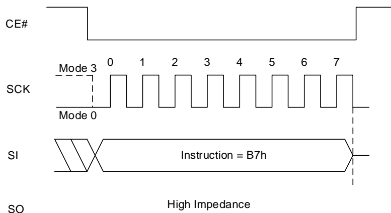
Figure 8.112 Enter 4-byte Address Mode Sequence
