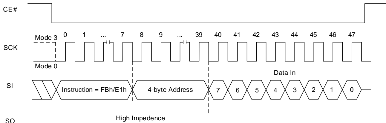
Figure 8.121 Write DYB Sequence (FBh [EXTADD=1] or E1h, 4-byte address)
