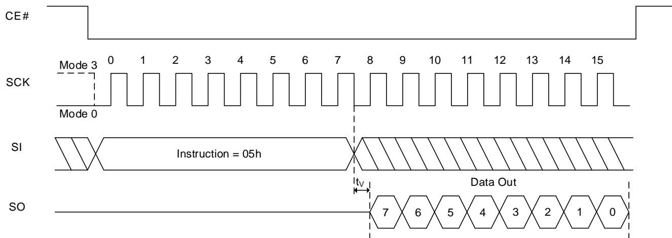
Figure 8.45 Read Status Register Sequence
