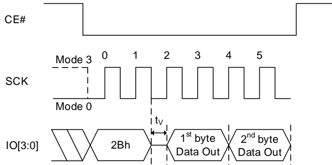
Figure 8.133 Read ASP QPI Sequence
