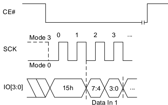
Figure 8.107 WRABR QPI Sequence (QE = 1)
