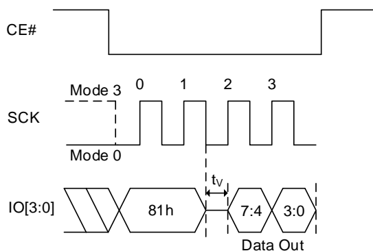
Figure 8.66 Read Extended Read Parameters QPI Sequence
