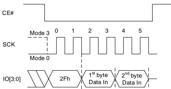
Figure 8.135 Program ASP QPI Sequence
