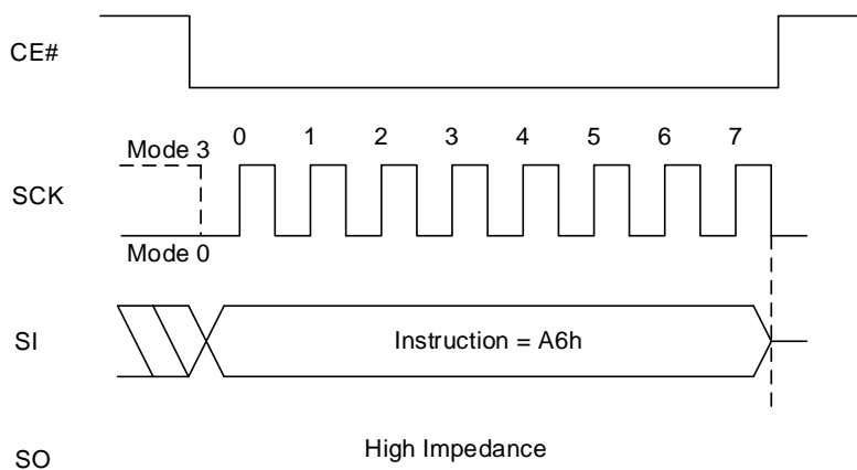
Figure 8.140 Set FREEZE Bit Sequence
