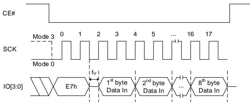
Figure 8.143 Read Password QPI Sequence
