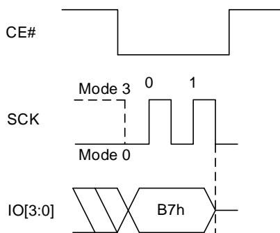
Figure 8.113 Enter 4-byte Address Mode QPI Sequence
