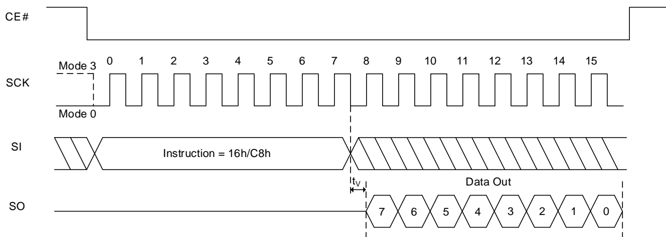
Figure 8.108 Read Bank Address Register Sequence
