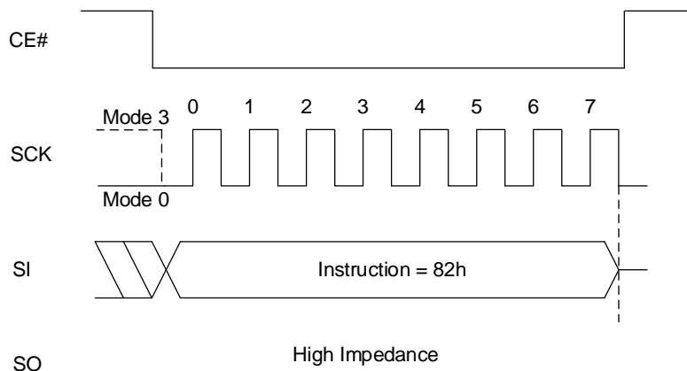
Figure 8.67 Clear Extended Read Register Sequence
