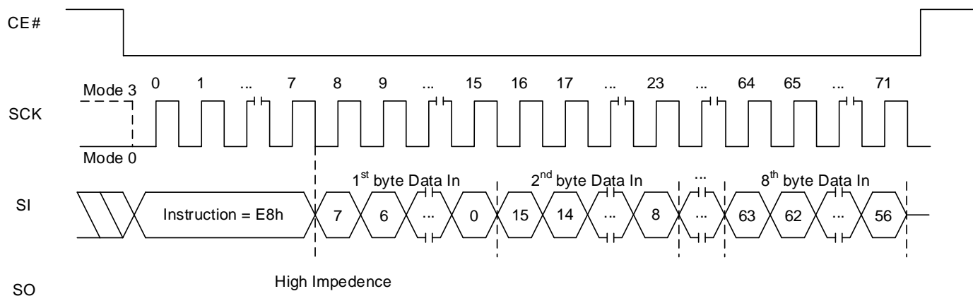
Figure 8.144 Program Password Sequence
