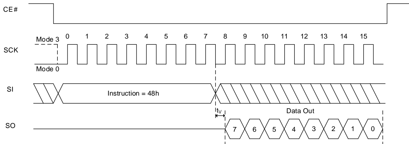
Figure 8.49 Read Function Register Sequence
