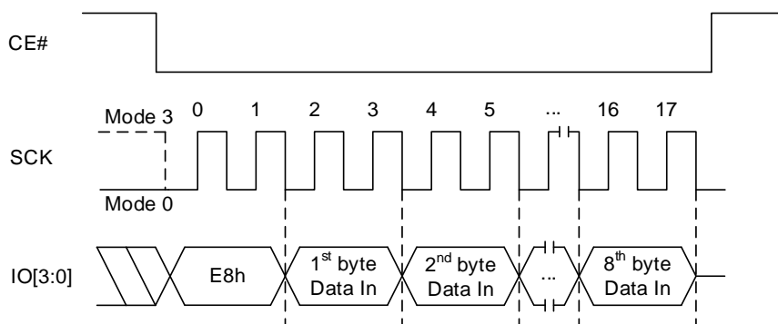
Figure 8.145 Program Password QPI Sequence
