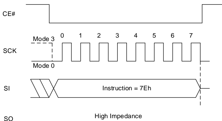
Figure 8.148 Gang Sector/Block Lock Sequence
