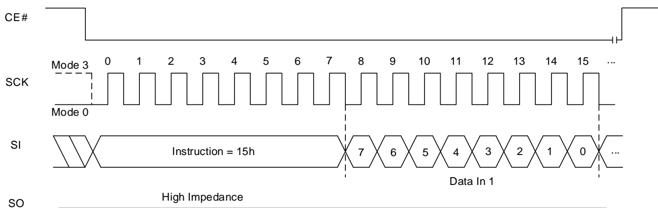
Figure 8.106 WRABR Sequence (QE = 1)
