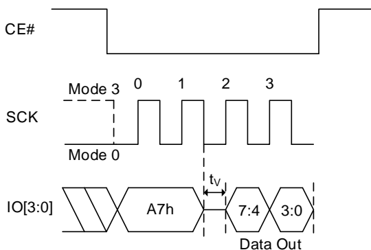
Figure 8.137 Read PPB Lock Bit QPI Sequence
