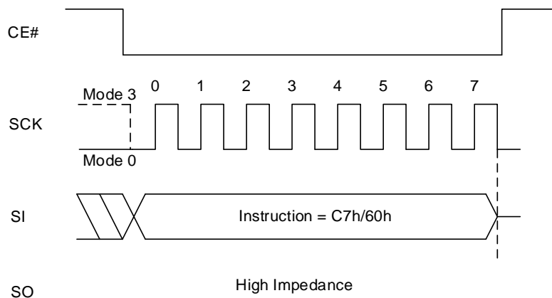
Figure 8.39 Chip Erase Sequence
