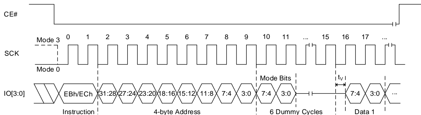
Figure 8.20 Fast Read Quad I/O QPI Sequence (EBh [EXTADD=1] or ECh, 4-byte address)
