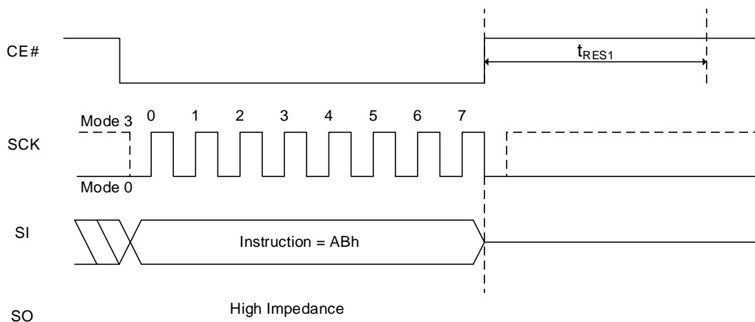
Figure 8.57 Release Power Down Mode Sequence
