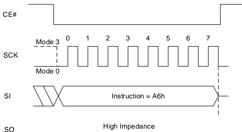
Figure 8.138 Write PPB Lock Bit Sequence
