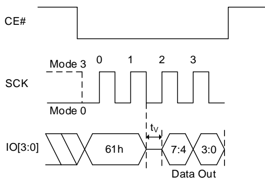
Figure 8.64 Read Read Parameters QPI Sequence
