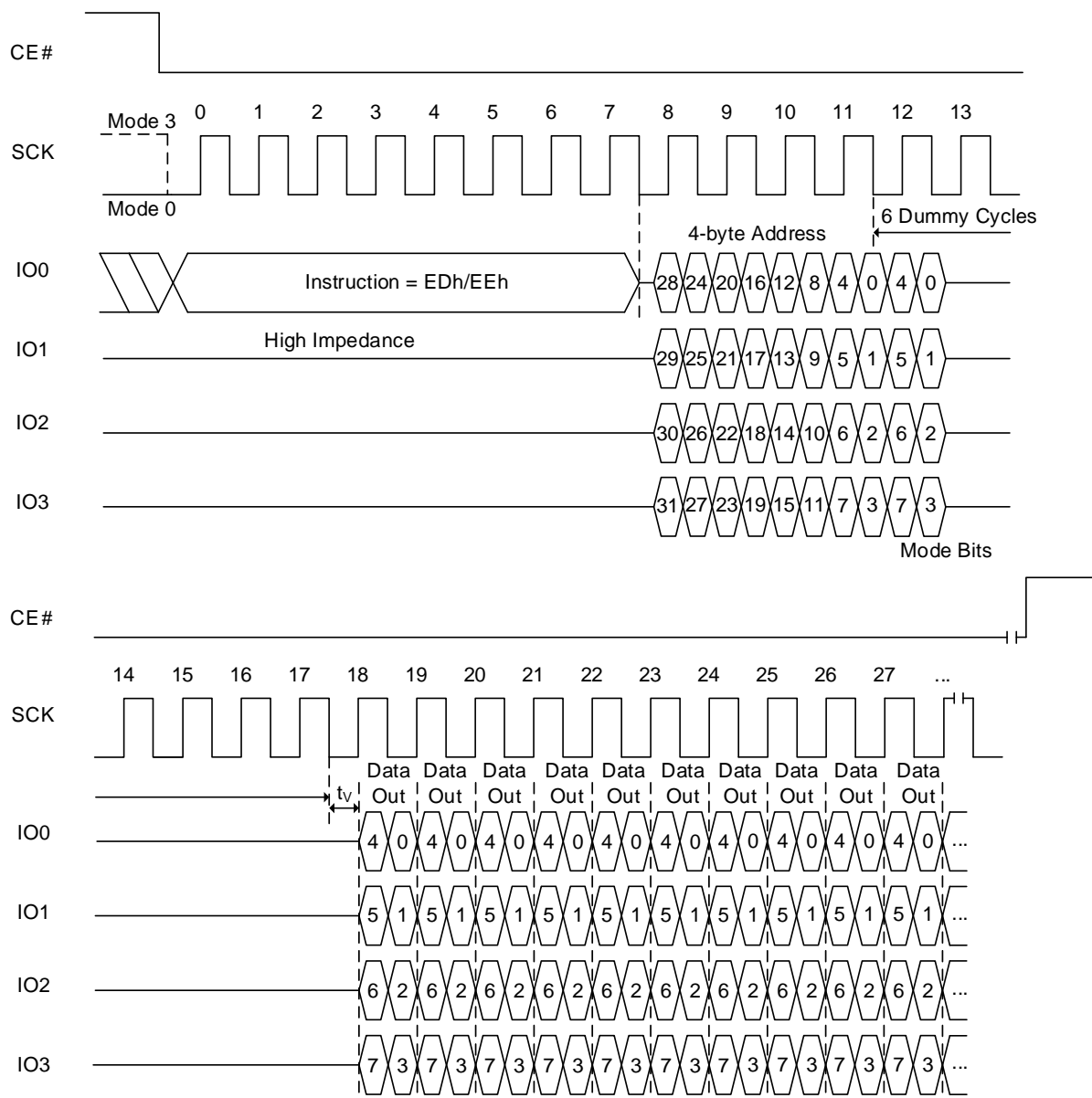
Figure 8.91 FRQDTR Sequence (EDh [EXTADD=1] or EEh, 4-byte address)
