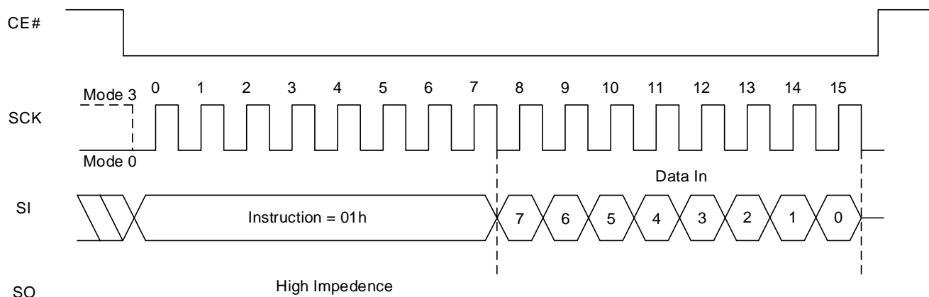
Figure 8.47 Write Status Register Sequence
