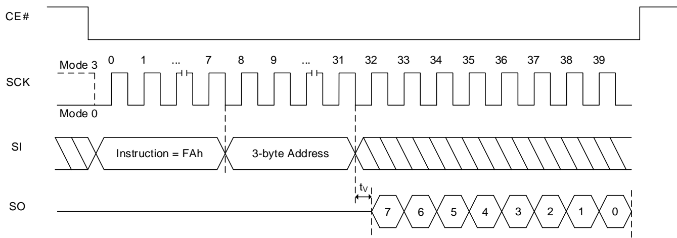
Figure 8.116 Read DYB Sequence (FAh [EXTADD=0], 3-byte address)
