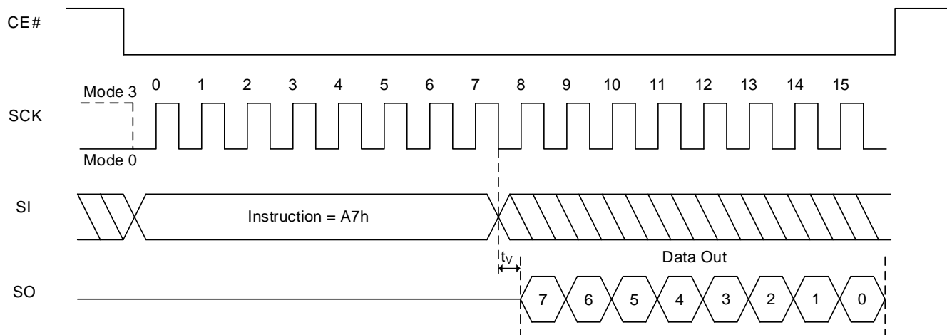
Figure 8.136 Read PPB Lock Bit Sequence
