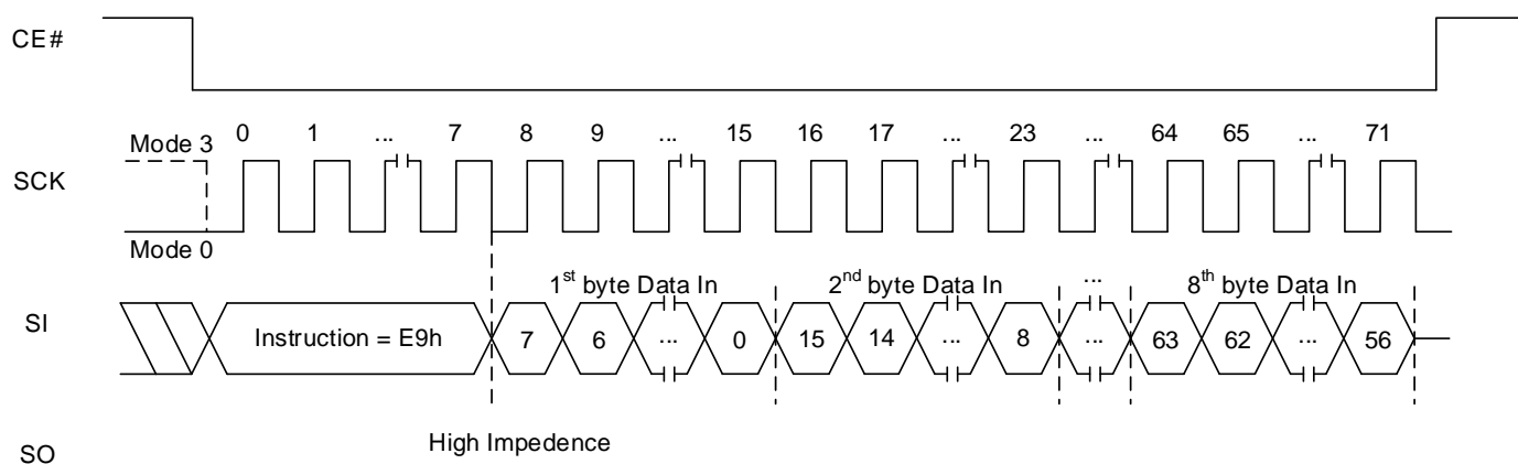
Figure 8.146 Unlock Password Sequence
