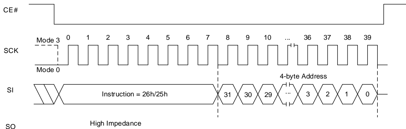
Figure 8.97 Sector Unlock Sequence (26h [EXTADD=1] or 25h, 4-byte address)
