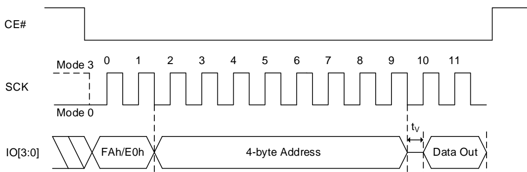
Figure 8.119 Read DYB QPI Sequence (FAh [EXTADD=0] or E0h, 4-byte address)
