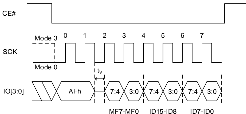
Figure 8.72 RDJDIDQ (Read JEDEC ID in QPI Mode) Sequence
