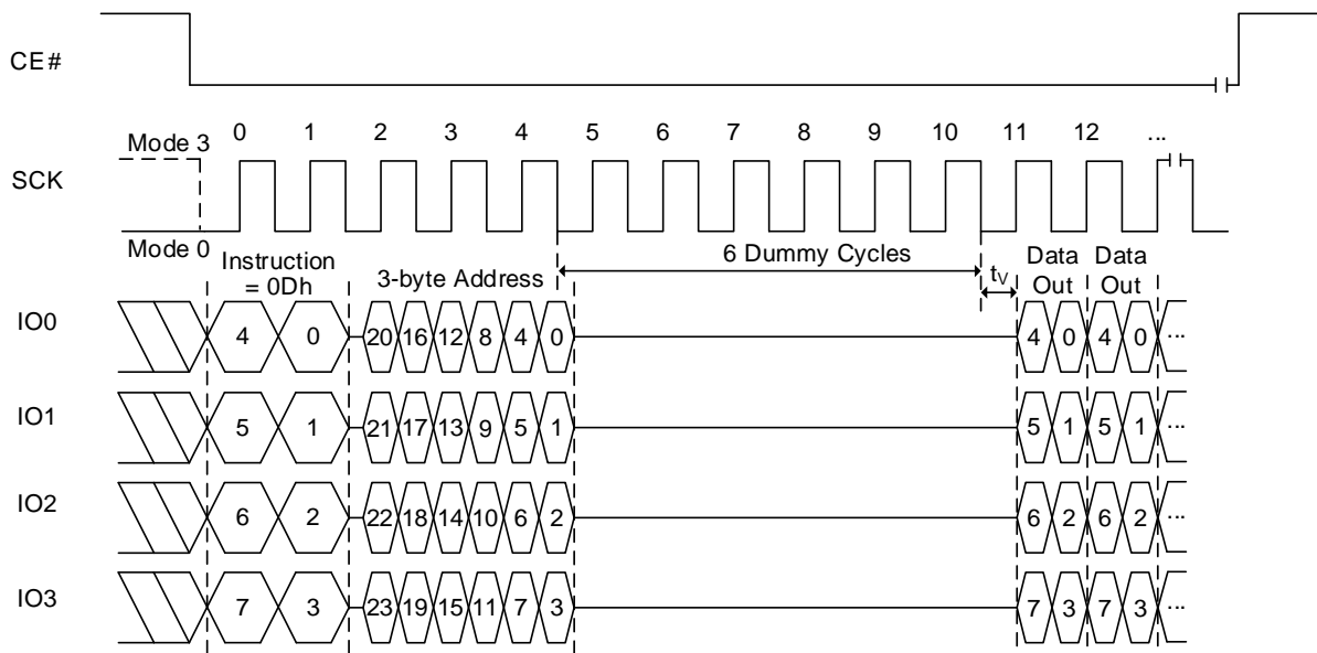
Figure 8.84 FRDTR QPI Sequence (0Dh [EXTADD=0], 3-byte address)
