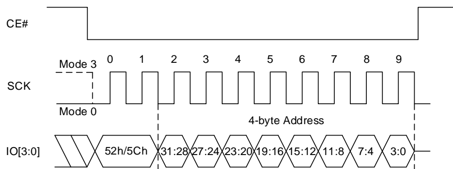
Figure 8.38 Block Erase (32K) QPI Sequence (52h [EXTADD=1] or 5Ch, 4-byte address)
