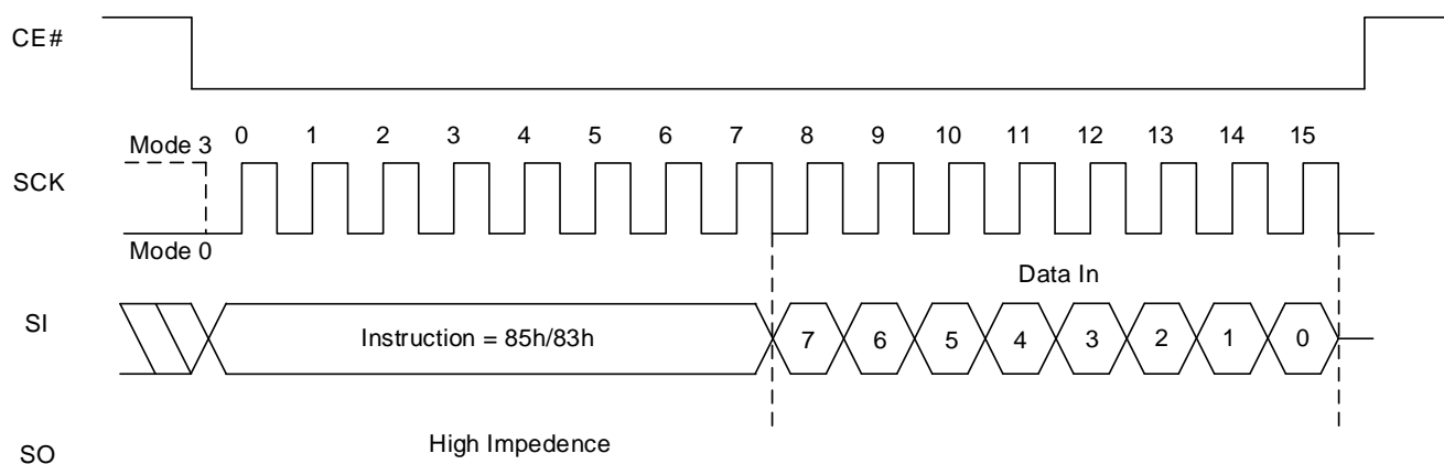
Figure 8.61 Set Extended Read Parameters Sequence
