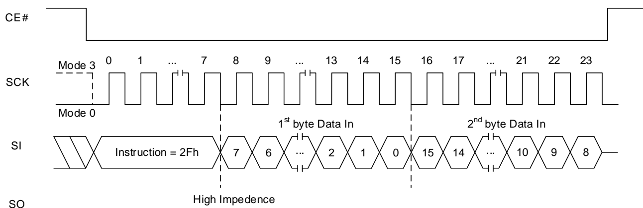
Figure 8.134 Program ASP Sequence
