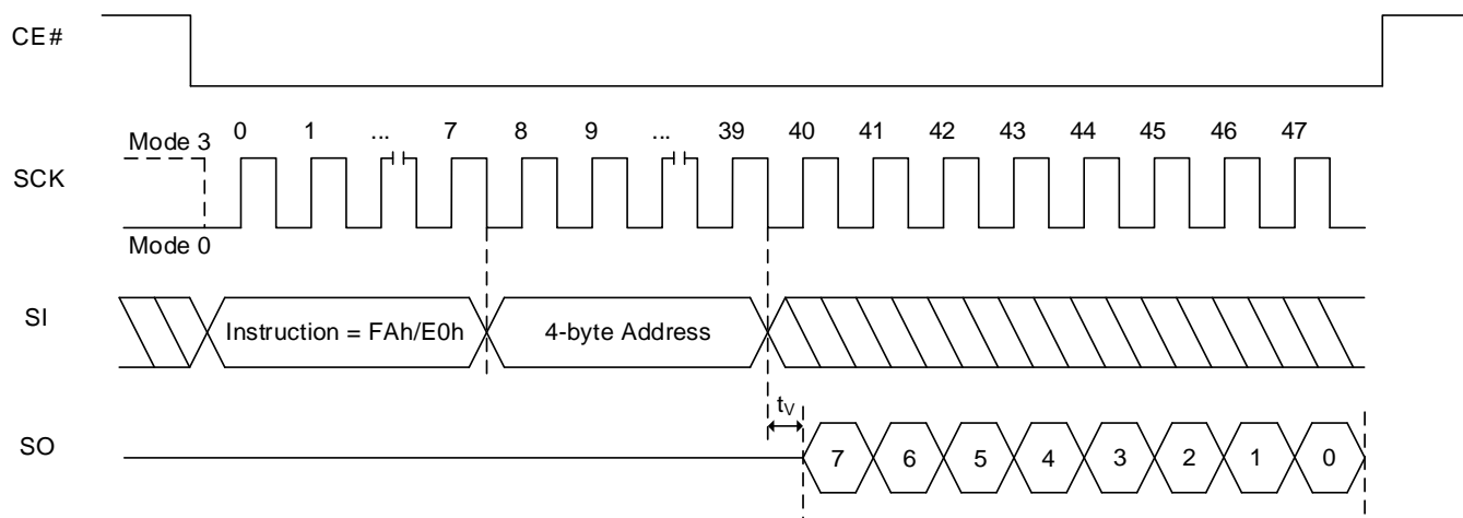
Figure 8.118 Read DYB QPI Sequence (FAh [EXTADD=0], 3-byte address)
