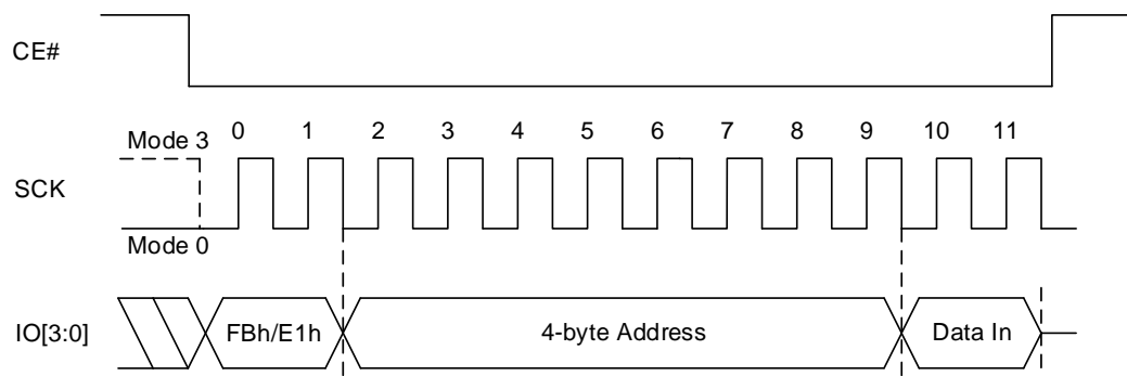
Figure 8.123 Write DYB QPI Sequence (FBh [EXTADD=1] or E1h, 4-byte address)
