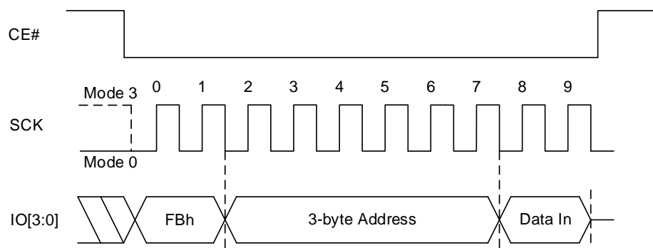
Figure 8.122 Write DYB QPI Sequence (FBh [EXTADD=0], 3-byte address)
