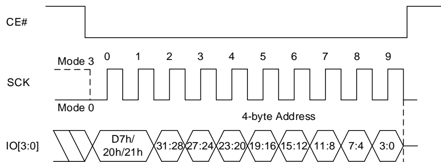
Figure 8.30 Sector Erase QPI Sequence (D7h/20h [EXTADD=1] or 21h, 4-byte address)
