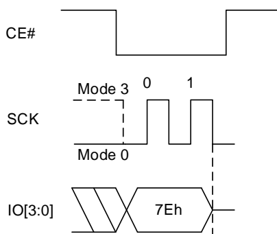
Figure 8.149 Gang Sector/Block Lock QPI Sequence
