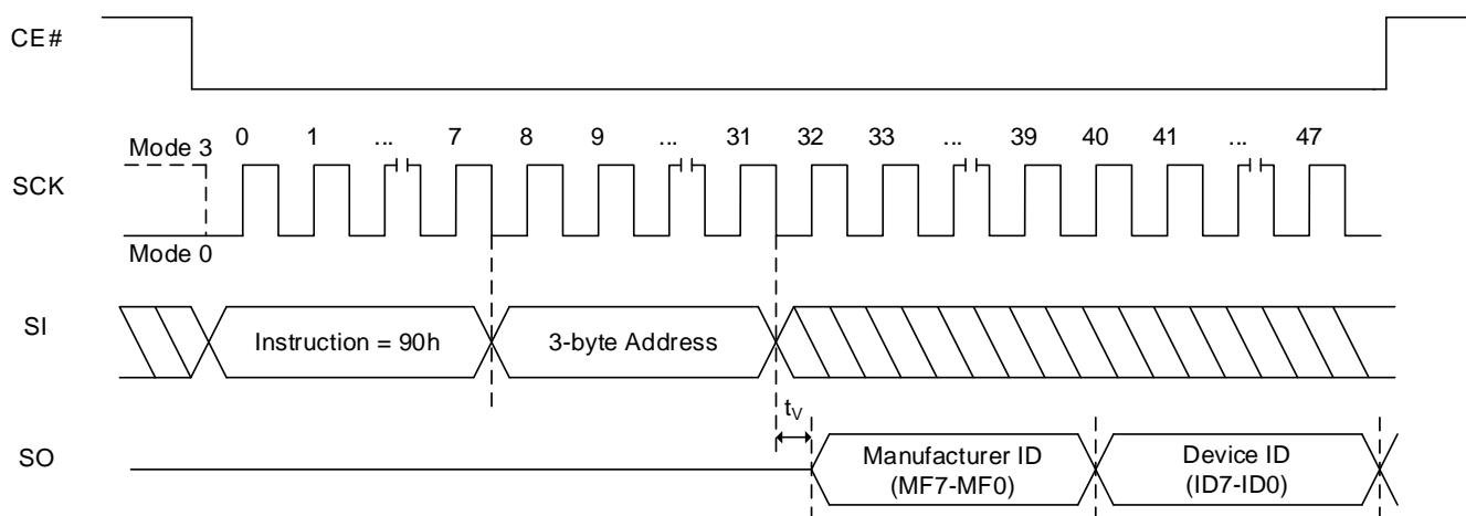
Figure 8.73 Read Product Identification by RDMDID Sequence
