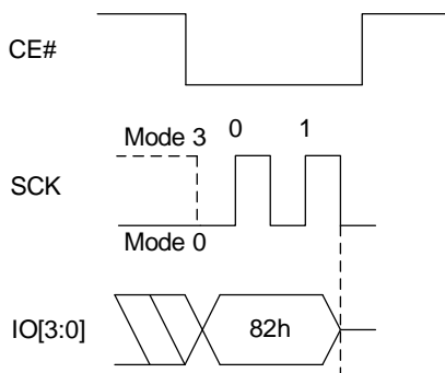
Figure 8.68 Clear Extended Read Register QPI Sequence
