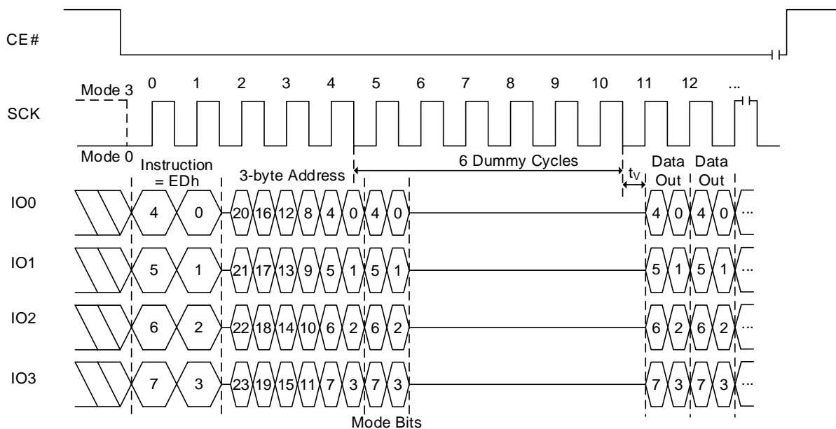
Figure 8.94 FRQDTR QPI Sequence (EDh [EXTADD=0], 3-byte address)
