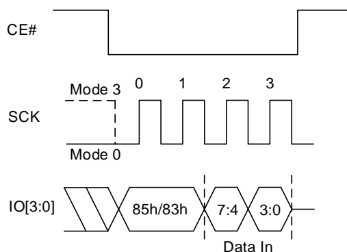
Figure 8.62 Set Extended Read Parameters QPI Sequence
