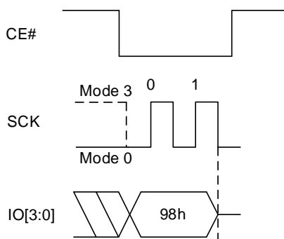
Figure 8.151 Gang Sector/Block Unlock QPI Sequence
