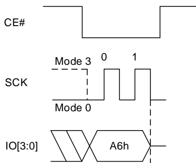
Figure 8.139 Write PPB Lock Bit QPI Sequence
