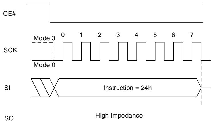
Figure 8.100 Sector Lock Sequence
