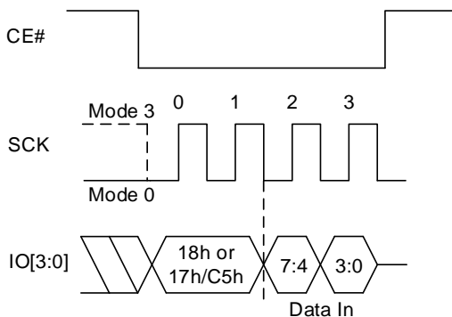
Figure 8.111 Write Bank Address Register QPI Sequence
