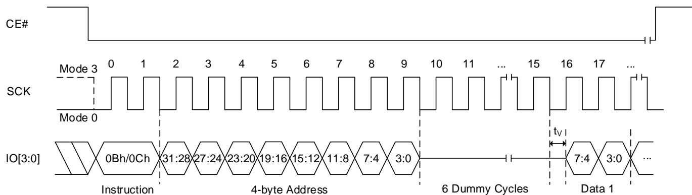
Figure 8.6 Fast Read QPI Sequence (0Bh [EXTADD=1] or 0Ch, 4-byte address)
