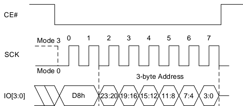
Figure 8.33 Block Erase (64K) QPI Sequence (D8h [EXTADD=0], 3-byte address)
