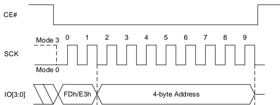
Figure 8.129 Program PPB QPI Sequence (FDh [EXTADD=1] or E3h, 4-byte address)
