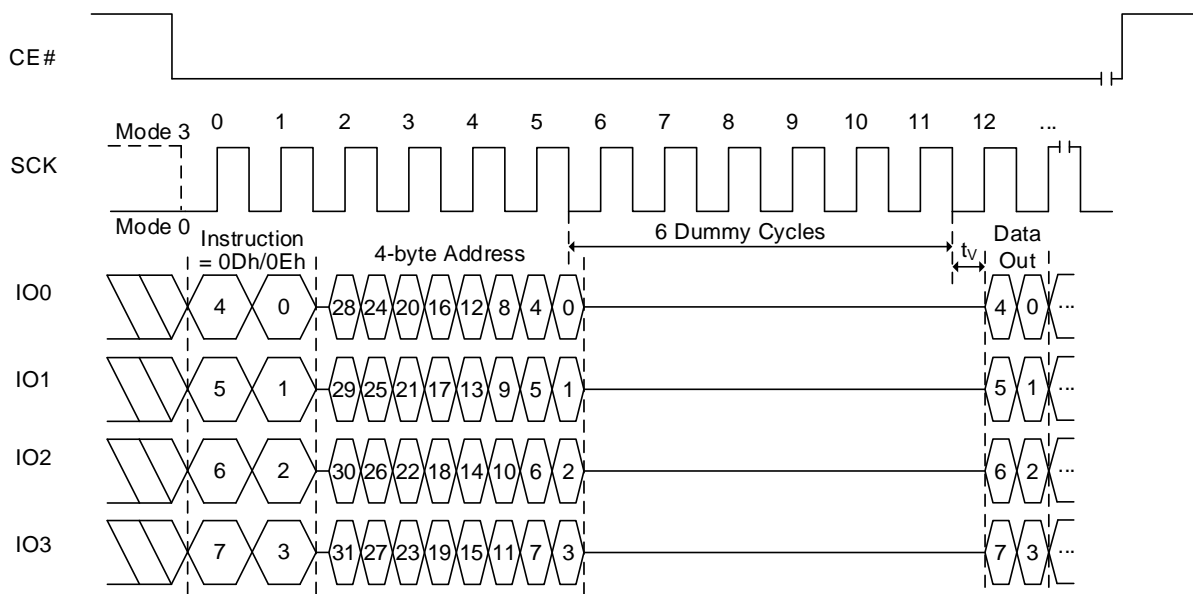
Figure 8.85 FRDTR QPI Sequence (0Dh [EXTADD=1] or 0Eh, 4-byte address)
