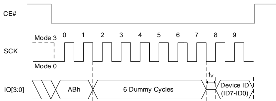
Figure 8.70 Read Product Identification QPI Sequence
