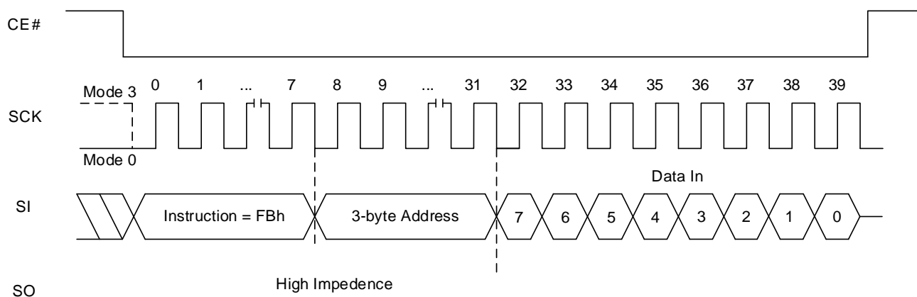
Figure 8.120 Write DYB Sequence (FBh [EXTADD=0], 3-byte address)
