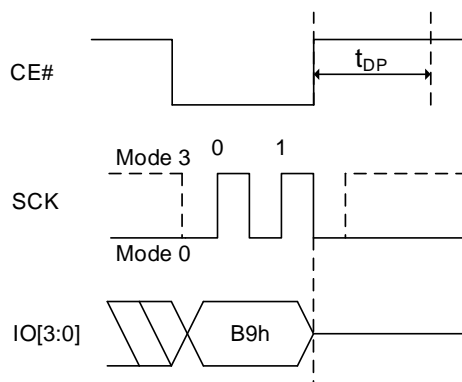
Figure 8.56 Enter Deep Power Down Mode QPI Sequence
