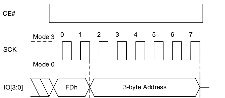
Figure 8.128 Program PPB QPI Sequence (FDh [EXTADD=0], 3-byte address)
