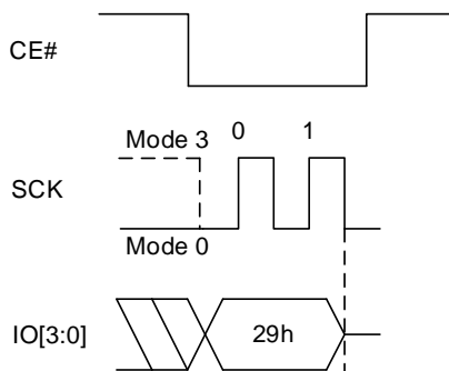
Figure 8.115 Exit 4-byte Address Mode QPI Sequence
