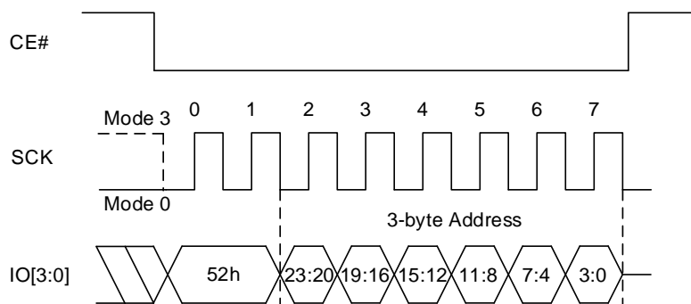
Figure 8.37 Block Erase (32K) QPI Sequence (52h [EXTADD=0], 3-byte address)
