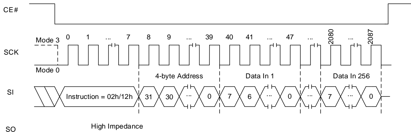
Figure 8.23 Page Program Sequence (02h [EXTADD=1] or 12h, 4-byte address)
