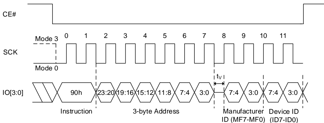
Figure 8.74 Read Product Identification by RDMDID QPI Sequence
