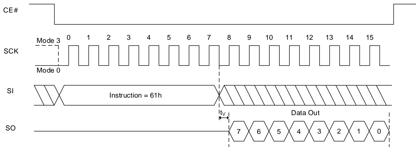
Figure 8.63 Read Read Parameters Sequence
