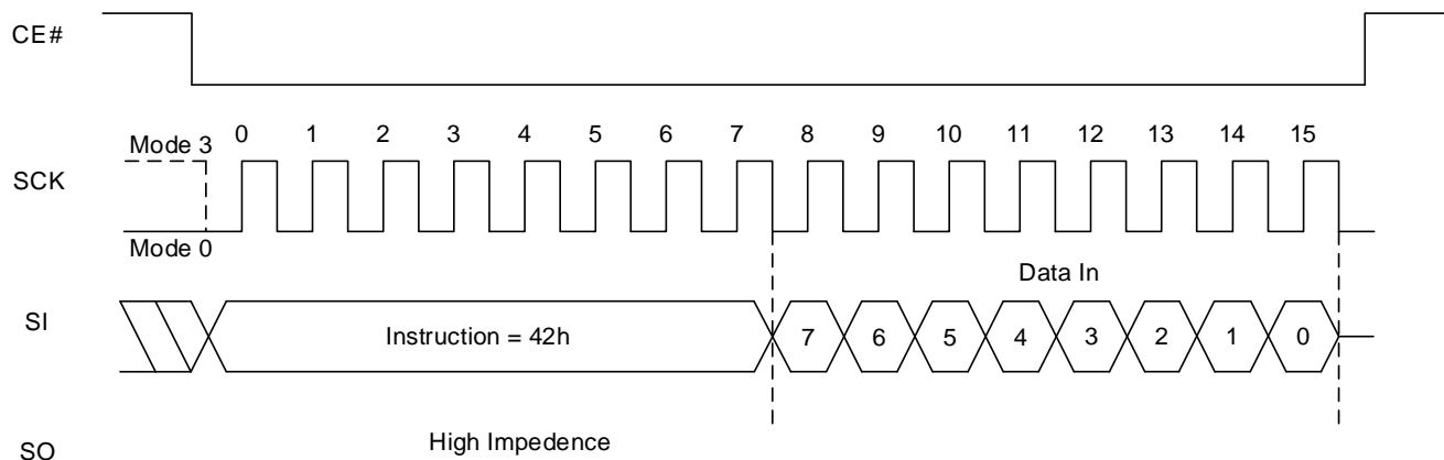
Figure 8.51 Write Function Register Sequence
