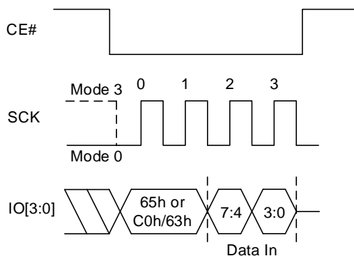
Figure 8.60 Set Read Parameters QPI Sequence
