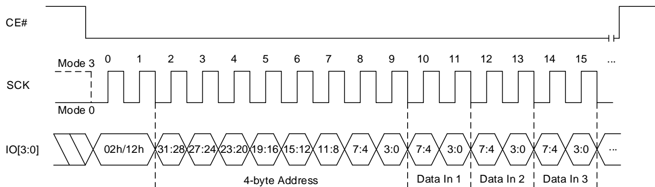
Figure 8.24 Page Program QPI Sequence (02h [EXTADD=1] or 12h, 4-byte address)
