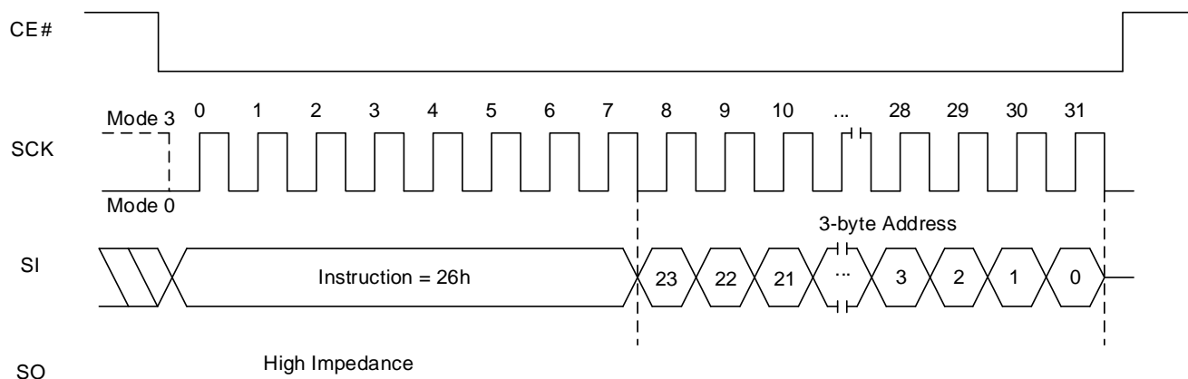
Figure 8.96 Sector Unlock Sequence (26h [EXTADD=0], 3-byte address)
