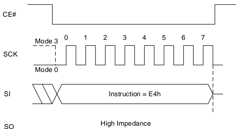
Figure 8.130 Erase PPB Sequence
