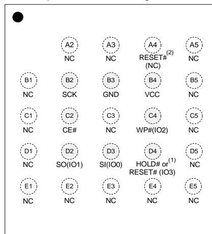
5x5 Ball Array
