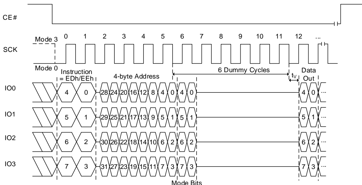
Figure 8.95 FRQDTR QPI Sequence (EDh [EXTADD=1] or EEh, 4-byte address)
