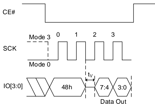
Figure 8.50 Read Function Register QPI Sequence
