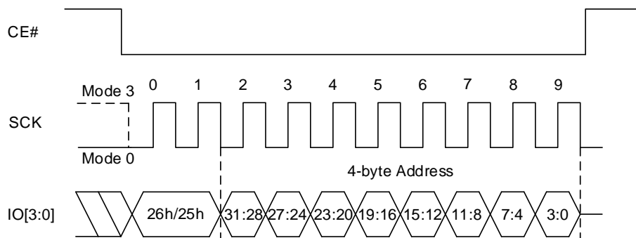
Figure 8.99 Sector Unlock QPI Sequence (26h [EXTADD=1] or 25h, 4-byte address)
