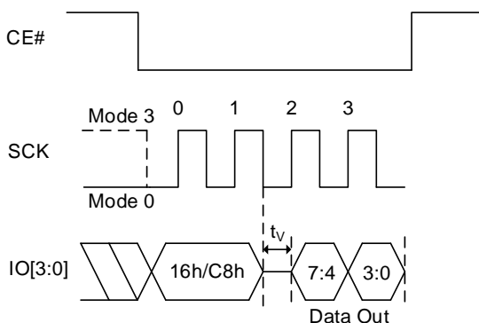
Figure 8.109 Read Bank Address Register QPI Sequence
