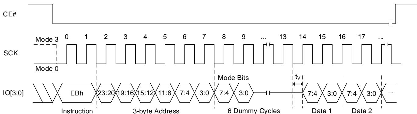
Figure 8.19 Fast Read Quad I/O QPI Sequence (EBh [EXTADD=0], 3-byte address)
