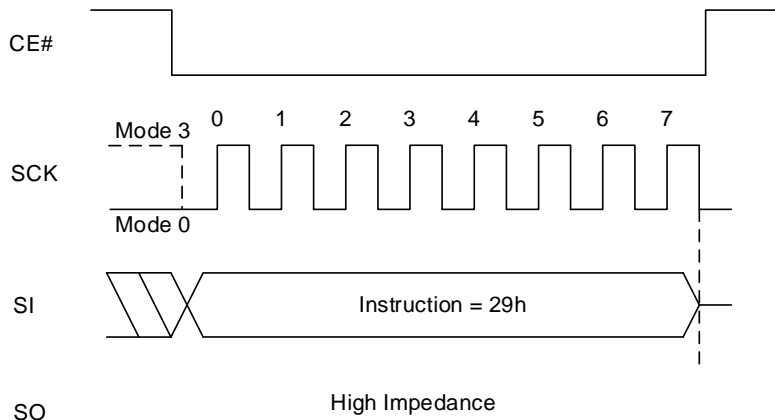
Figure 8.114 Exit 4-byte Address Mode Sequence
