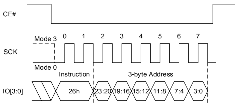
Figure 8.98 Sector Unlock QPI Sequence (26h [EXTADD=0], 3-byte address)
