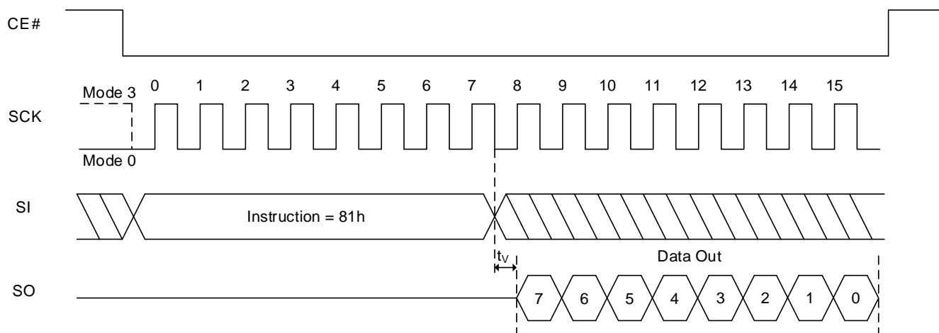
Figure 8.65 Read Extended Read Parameters Sequence
