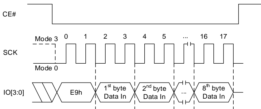
Figure 8.147 Unlock Password QPI Sequence
