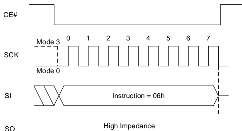
Figure 8.41 Write Enable Sequence
