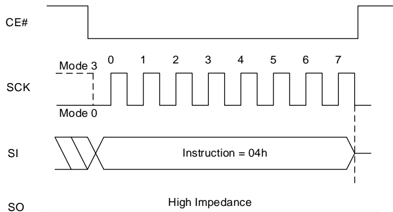
Figure 8.43 Write Disable Sequence
