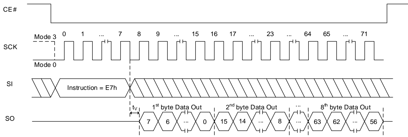
Figure 8.142 Read password Sequence
