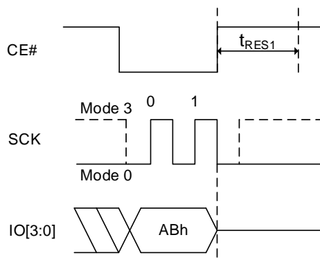
Figure 8.58 Release Power Down Mode QPI Sequence
