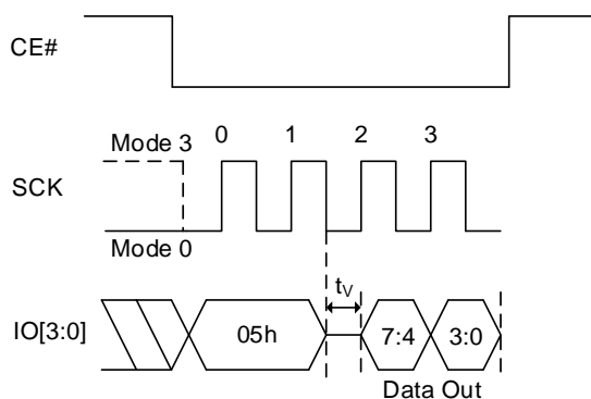
Figure 8.46 Read Status Register QPI Sequence
