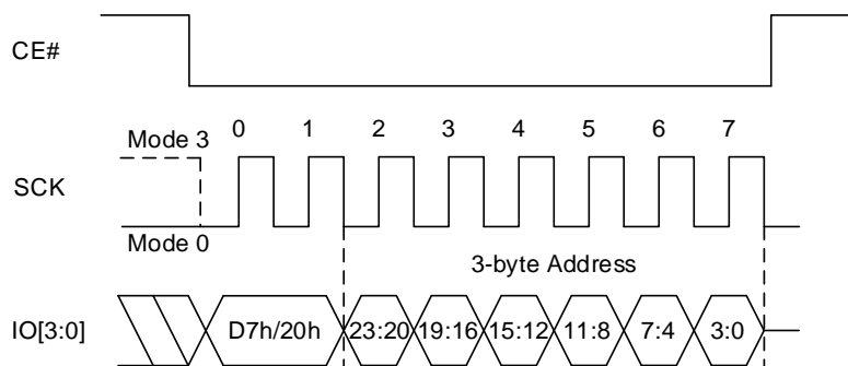
Figure 8.29 Sector Erase QPI Sequence (D7h/20h [EXTADD=0], 3-byte address)
