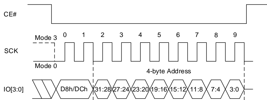
Figure 8.34 Block Erase (64K) QPI Sequence (D8h [EXTADD=1] or DCh, 4-byte address)
