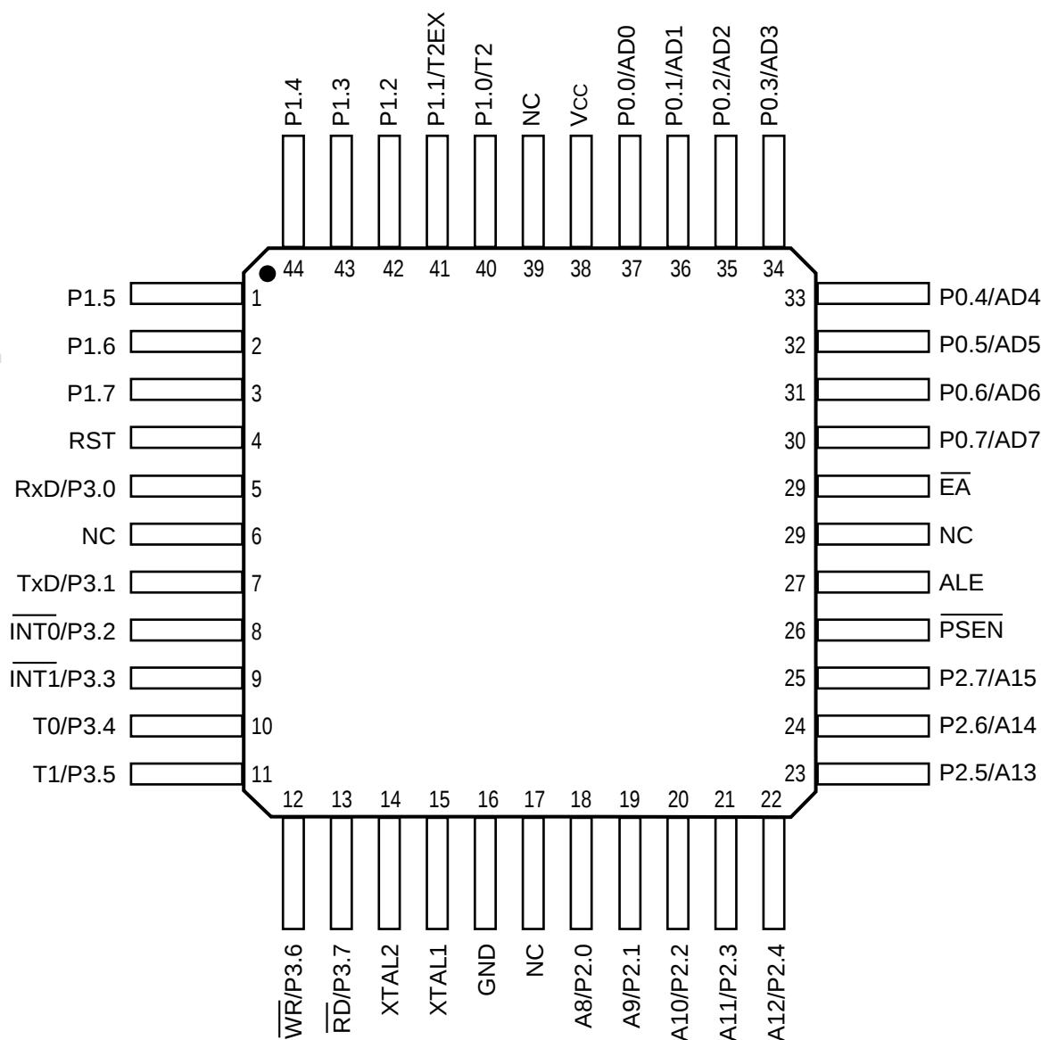
Figure 3. IS80C52/32 Pin Configuration: 44-pin PQFP
