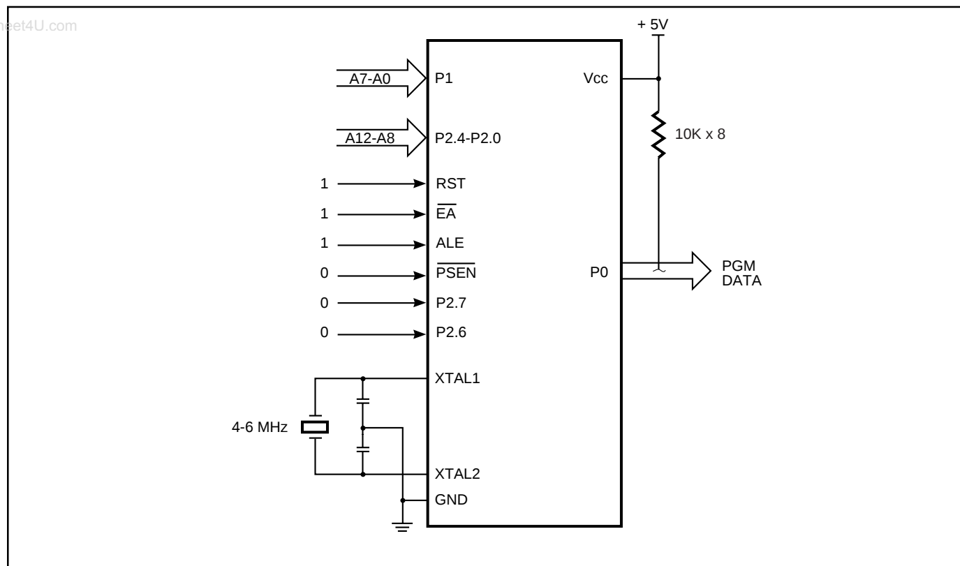
Figure 27. ROM Verification
