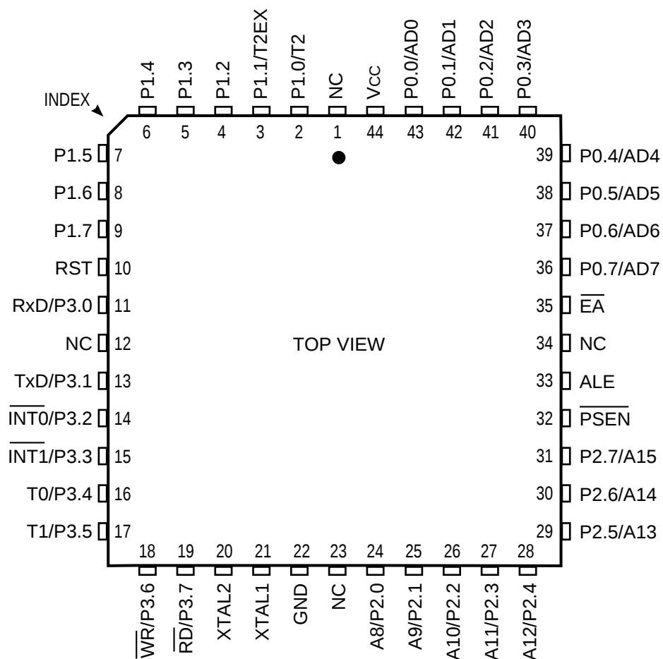
Figure 2. IS80C52/32 Pin Configuration: 44-pin PLCC
