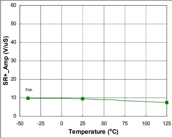
Fig. 48. Operational Amplifier Slew Rate (+) vs. Temperature
