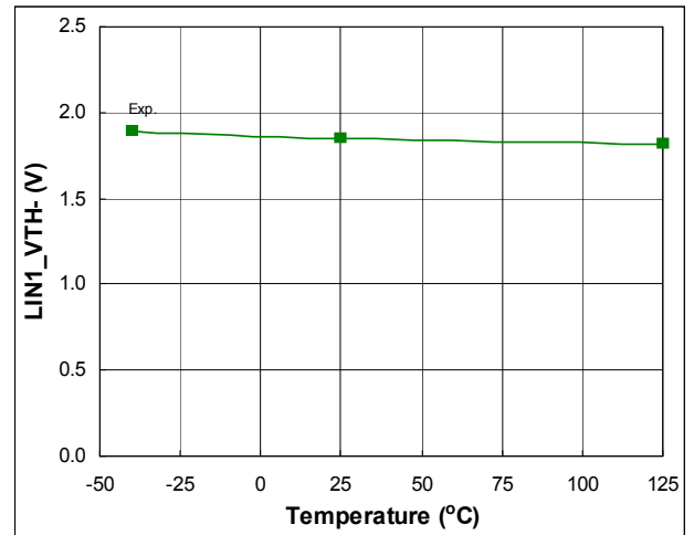
Fig. 53. Input Negative Going Threshold vs. Temperature
