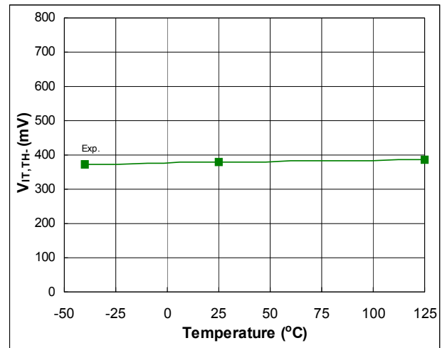
Fig. 55. ITRIP Input Negative Going Threshold vs. Temperature
