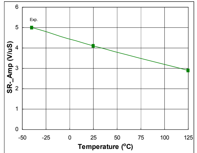
Fig. 51. Operational Amplifier Slew Rate (-) vs. Temperature
