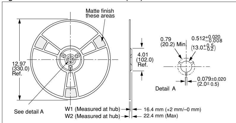
Figure 9. Reel Dimensions in Inches (mm)
