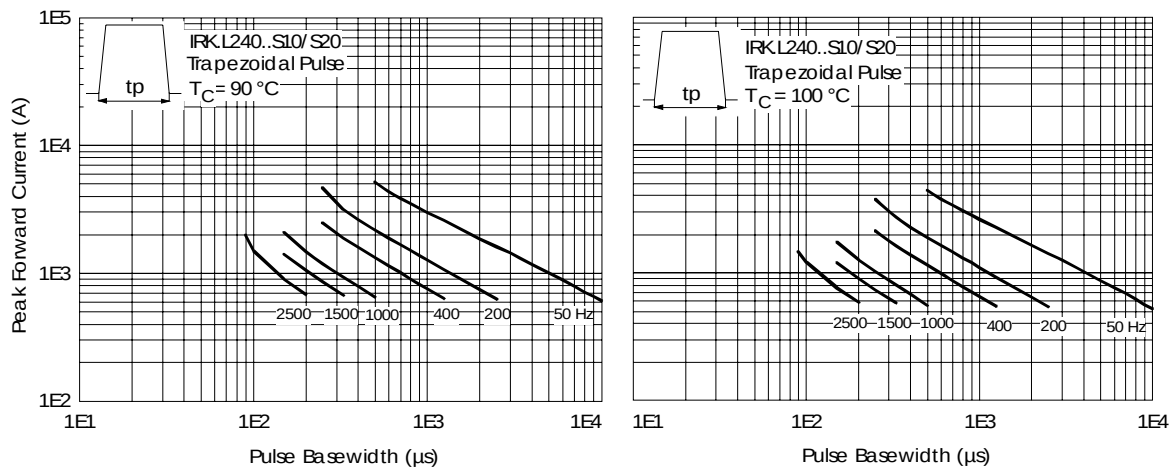
Fig. 23 - Frequency Characteristics
