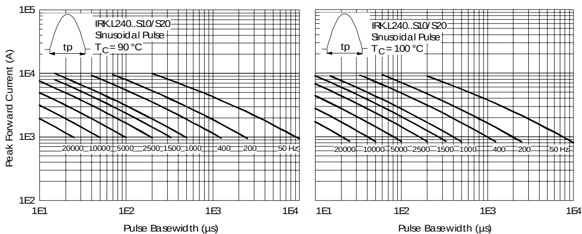
Fig. 22 - Frequency Characteristics
