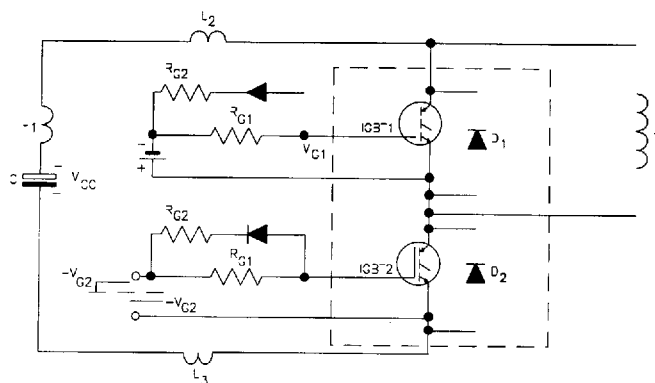
Fig. 16 - Test Circuit for Measurement of I_{LM} , E_{ON} , E_{OFF} , Q_{RR} , I_{RR} , t_{D(ON)} , t_r , t_{D(OFF)} , t_i
