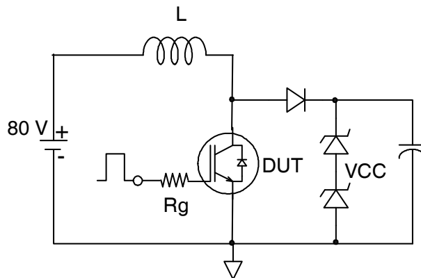
Fig.C.T.2 - RBSOA Circuit
