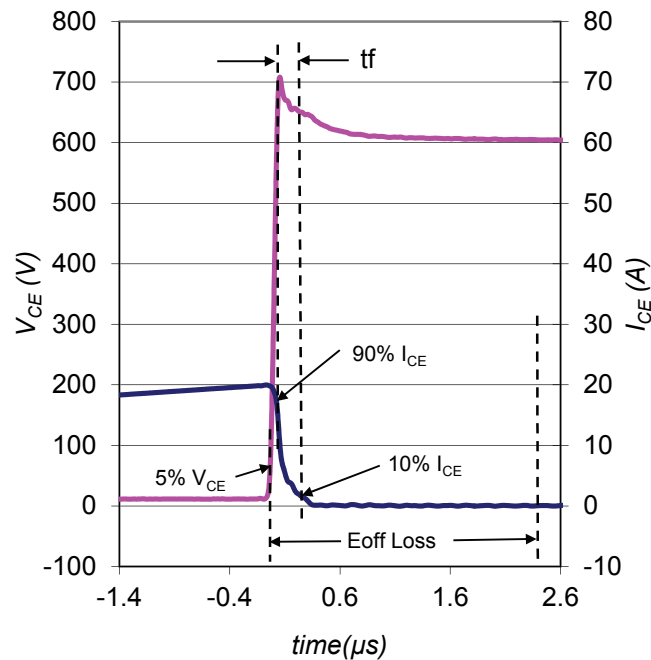
Fig. WF1 - Typ. Turn-off Loss Waveform @ T J = 150°C using Fig. CT.3
