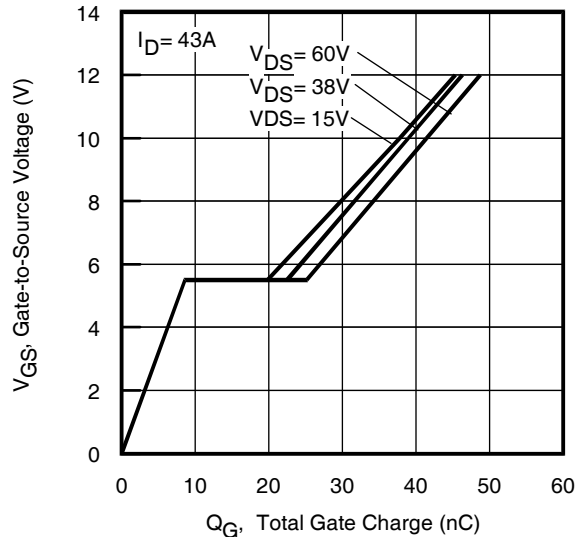
Fig 6. Typical Gate Charge Vs. Gate-to-Source Voltage www.DataSheet4U.com
