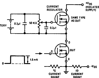
Fig. 18 - Gate Charge Test Circuit
