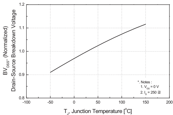
Fig 7. Breakdown Voltage Variation vs. Junction Temperature
