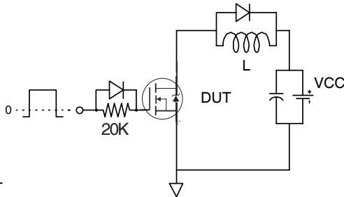
Fig 15. Gate Charge Test Circuit
