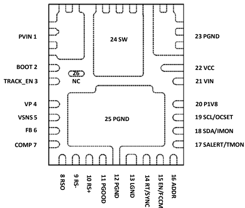
Figure 2: IR38060 package (Top View) 5mm x 6mm PQFN
