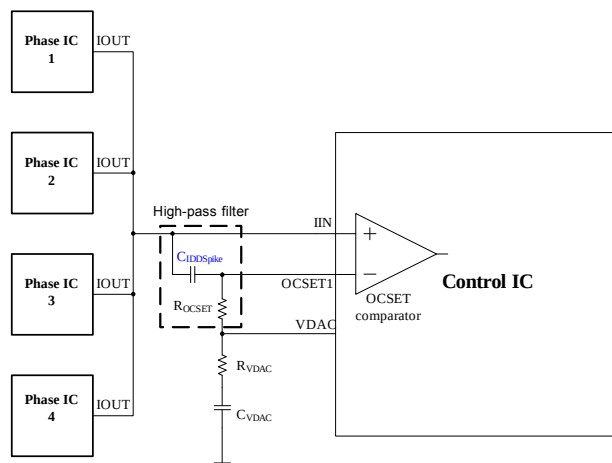
Figure 19 C_{IDD\text{Spike}} and R_{OCSET} form a High Pass Filter
