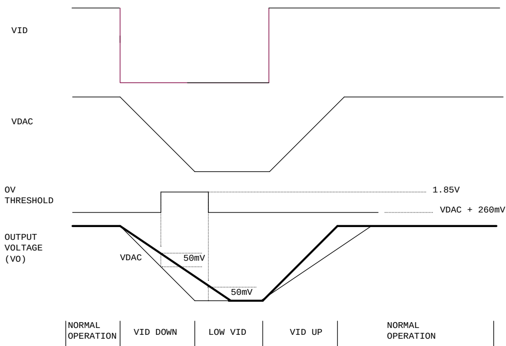
Figure 16 Over-voltage protection during dynamic VID
